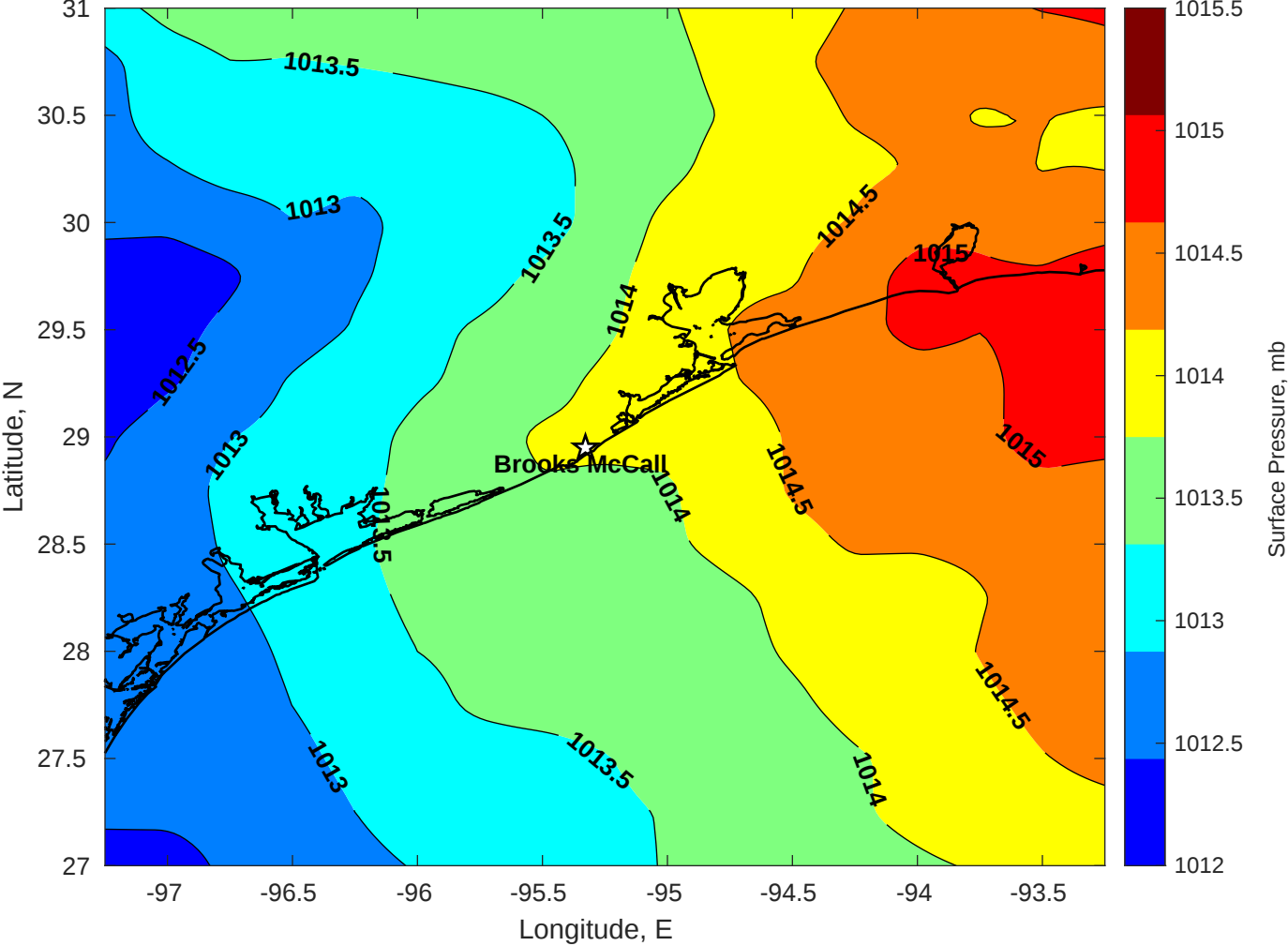
Surface Pressure (mb) for Brooks McCall at 22-Apr-2025 00:00:00
