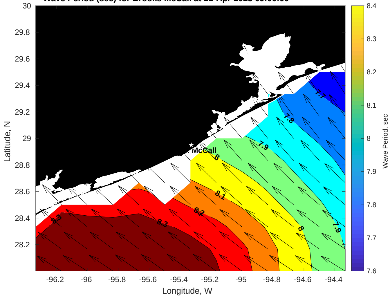
Wave Period (sec) for Brooks McCall at 21-Apr-2025 09:00:00
