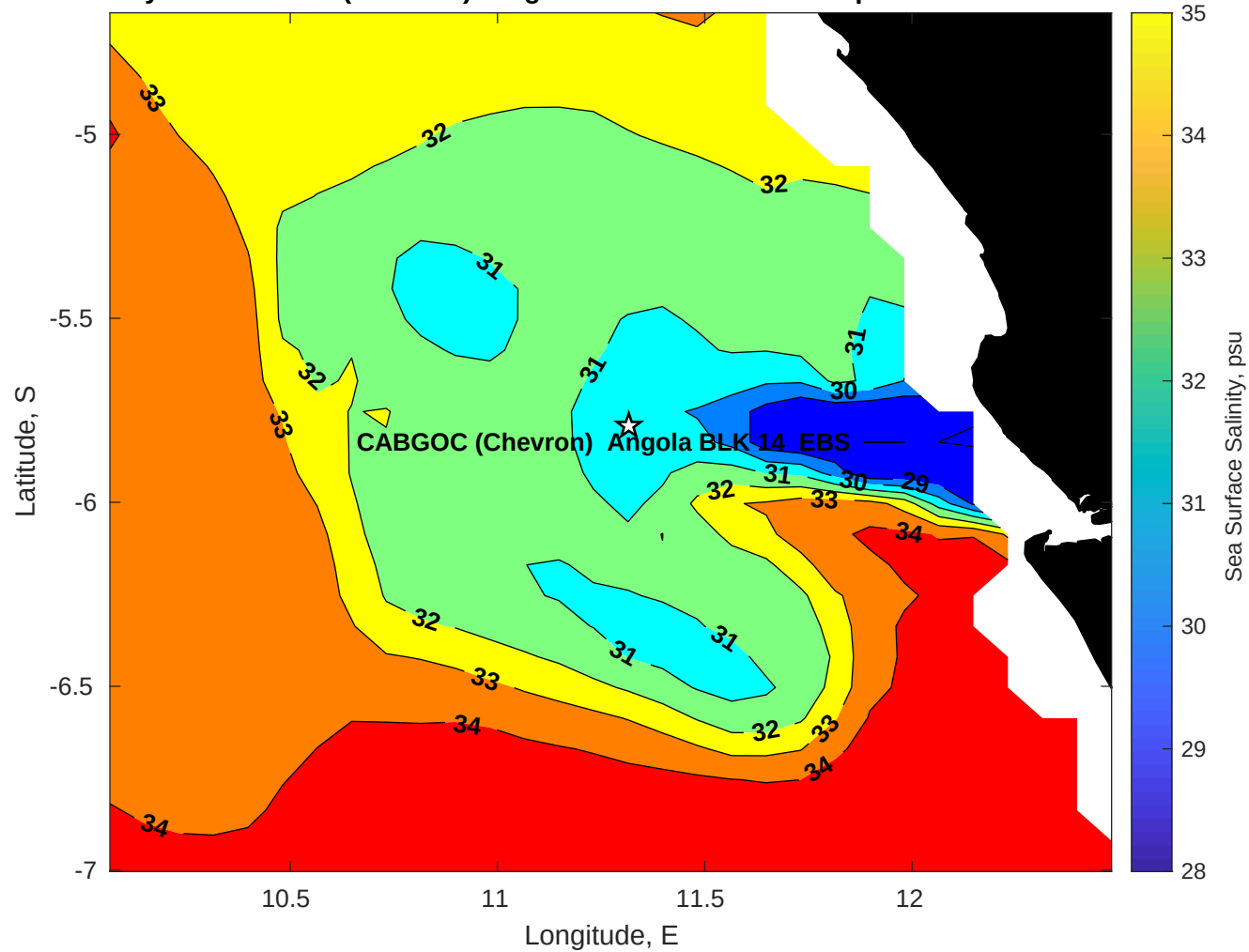
Surface Salinity for CABGOC (Chevron) Angola BLK 14 EBS at 20-Apr-2025 00:00:00
