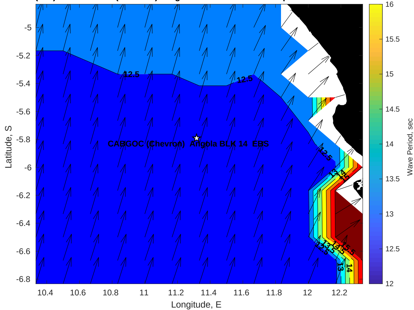
Wave Period (sec) for CABGOC (Chevron) Angola BLK 14 EBS at 21-Apr-2025 09:00:00
