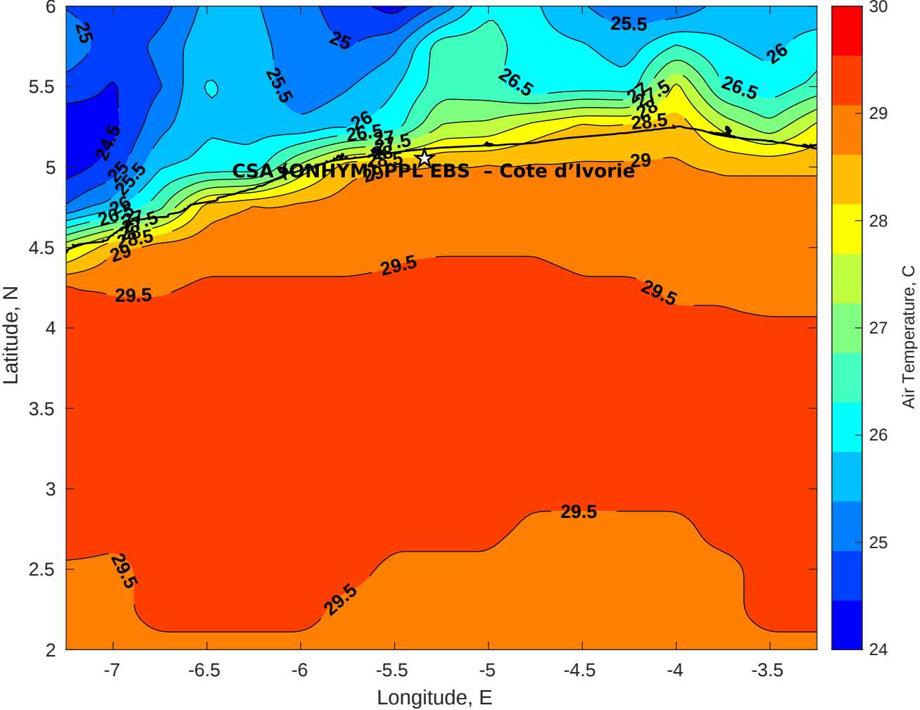
Air Temperature (C) for CSA (ONHYM) PPL EBS - Cote d'Ivoire at 21-Apr-2025
