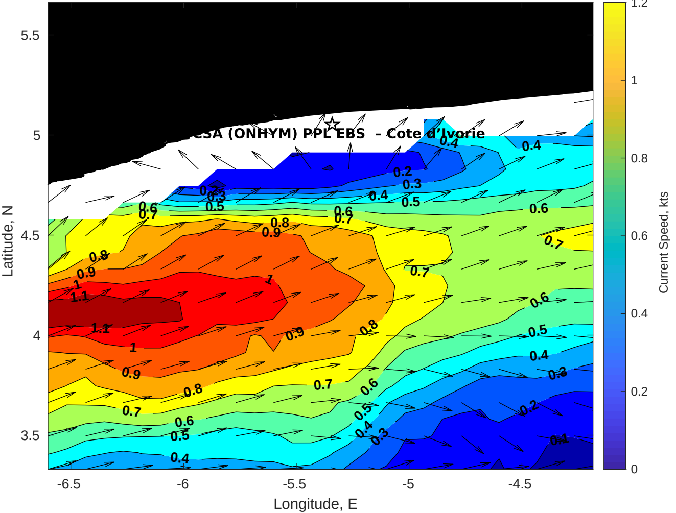
Surface Currents for CSA (ONHYM) PPL EBS - Cote d'Ivoire at 20-Apr-2025 00:00:00
