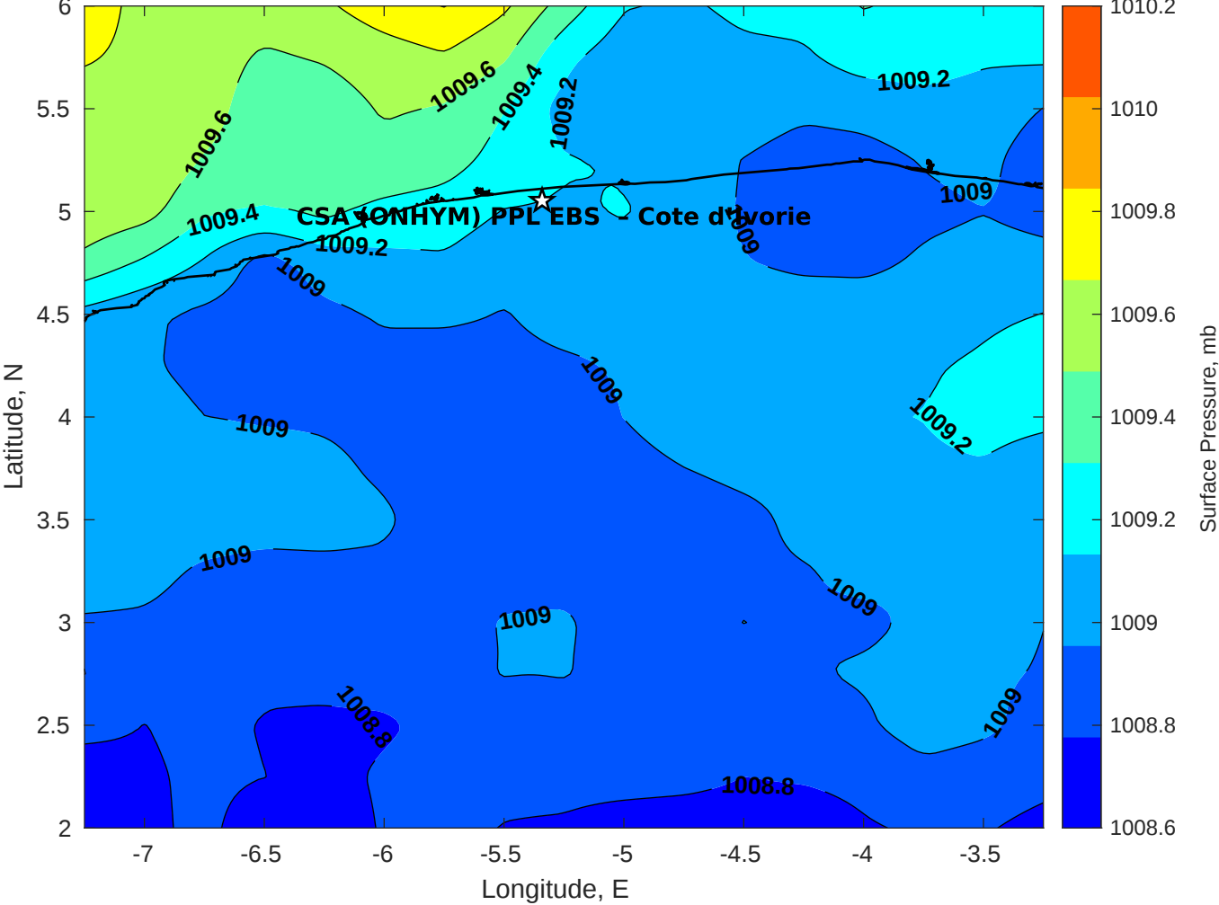
Surface Pressure (mb) for CSA (ONHYM) PPL EBS - Cote d'Ivoire at 21-Apr-2025 00:00:00
