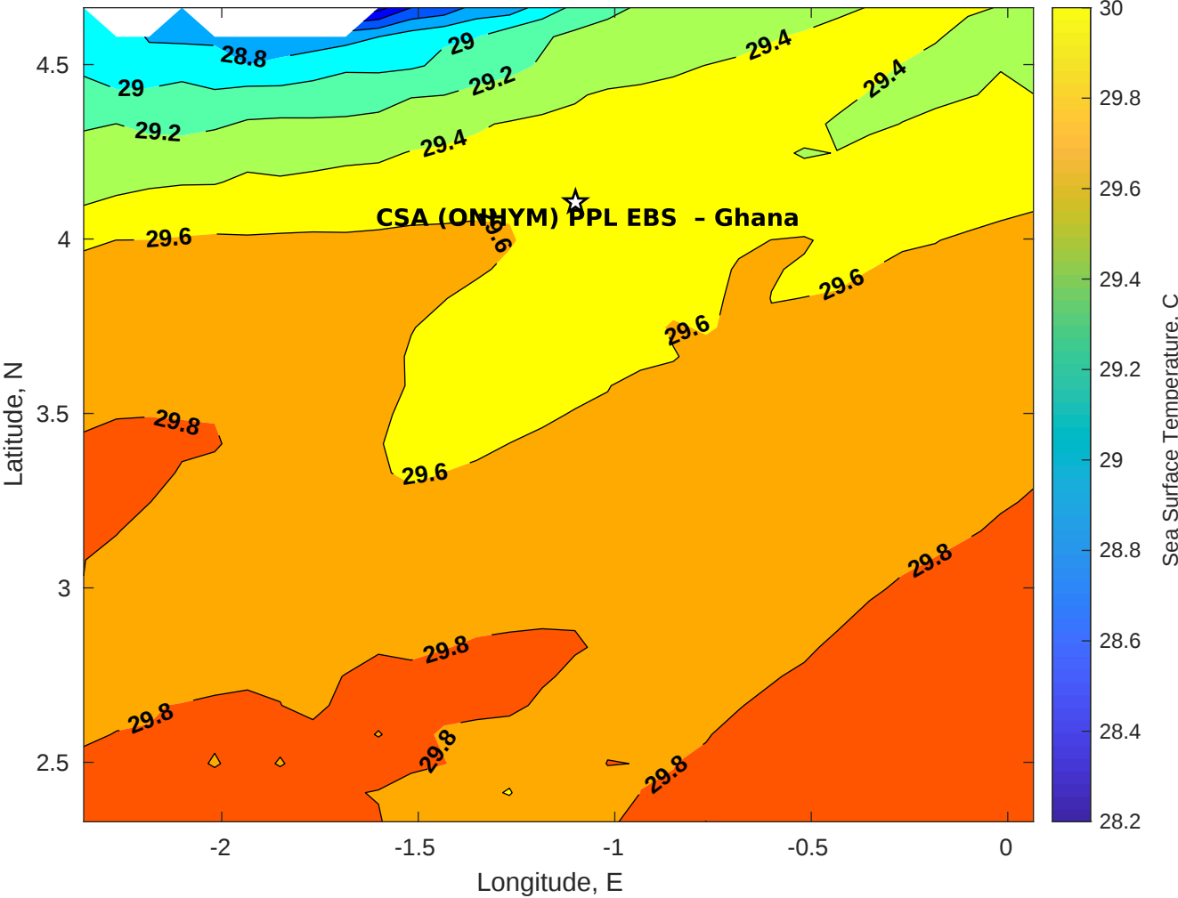
SST for CSA (ONHYM) PPL EBS - Ghana at 20-Apr-2025 00:00:00
