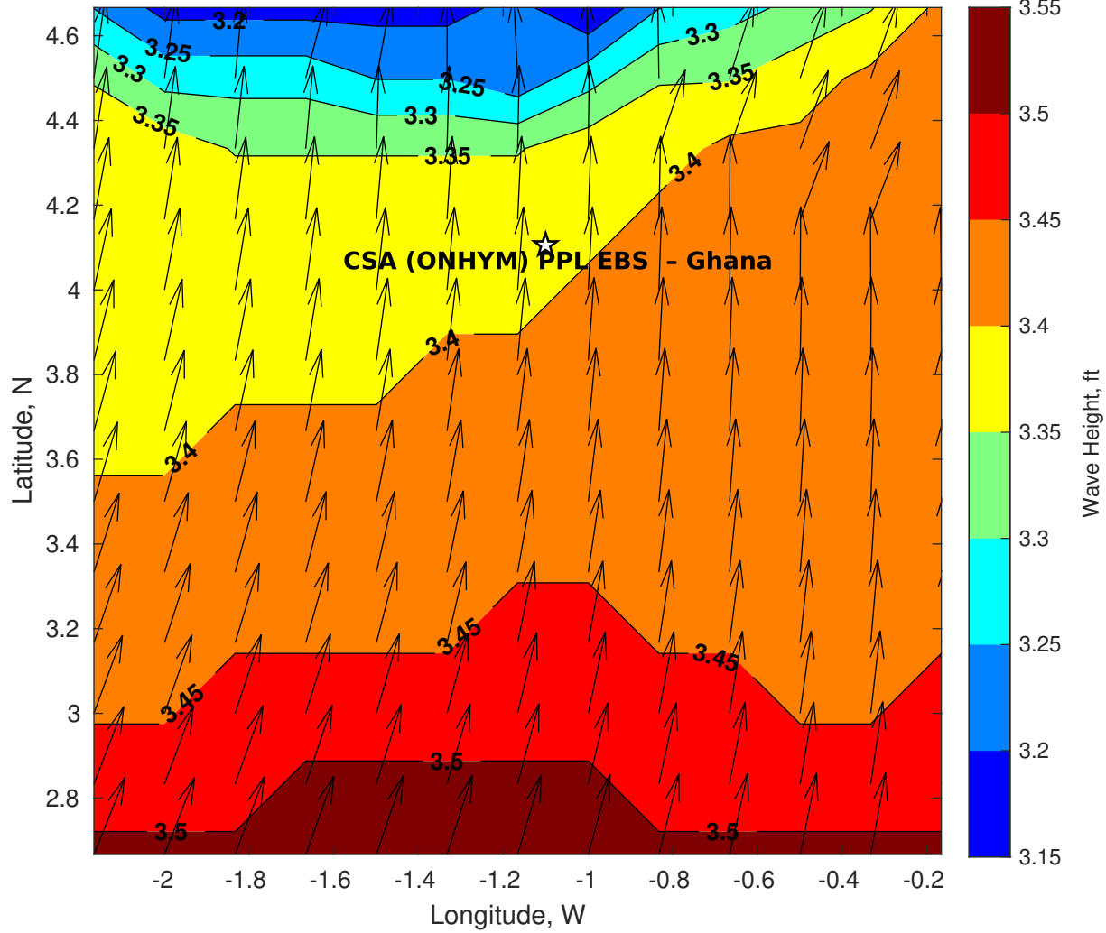
Wave Height (ft) for CSA (ONHYM) PPL EBS - Ghana at 21-Apr-2025 09:00:00
