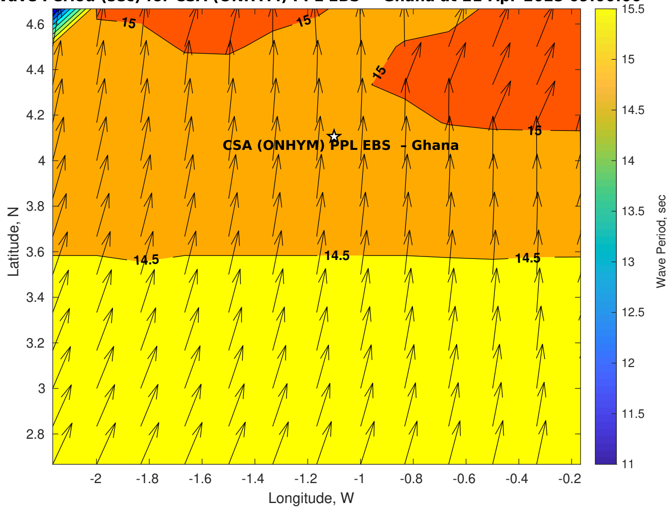
Wave Period (sec) for CSA (ONHYM) PPL EBS - Ghana at 21-Apr-2025 09:00:00
