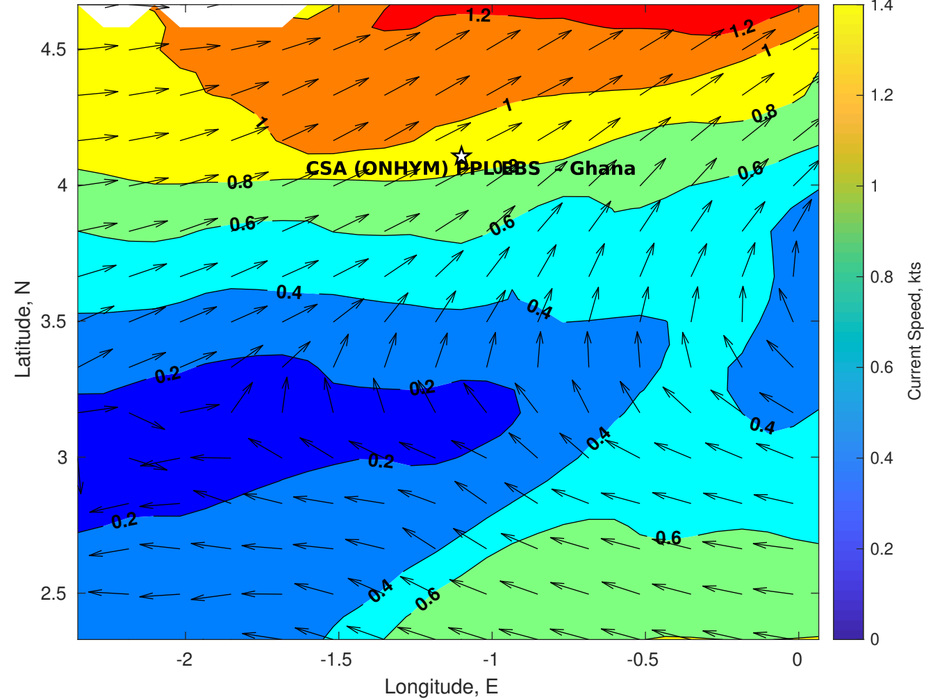
Surface Currents for CSA (ONHYM) PPL EBS - Ghana at 20-Apr-2025 00:00:00
