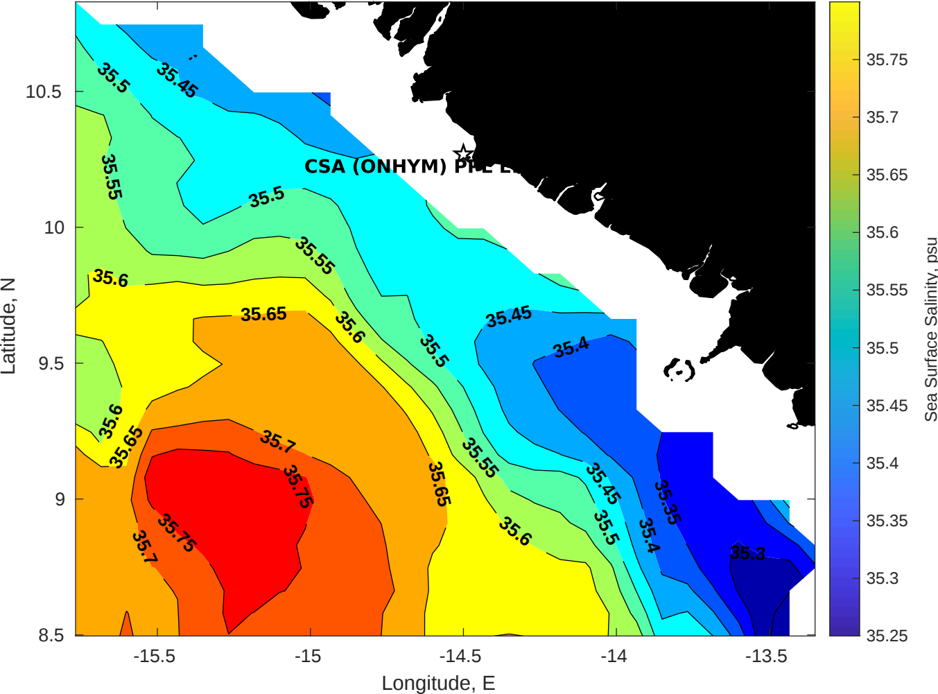
Surface Salinity for CSA (ONHYM) PPL EBS - Guinea at 20-Apr-2025 00:00:00
