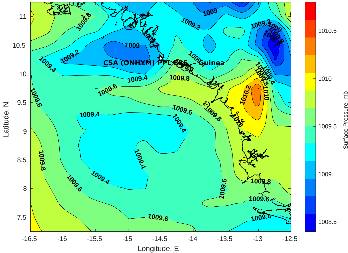
Surface Pressure (mb) for CSA (ONHYM) PPL EBS - Guinea at 21-Apr-2025 00:00:00
