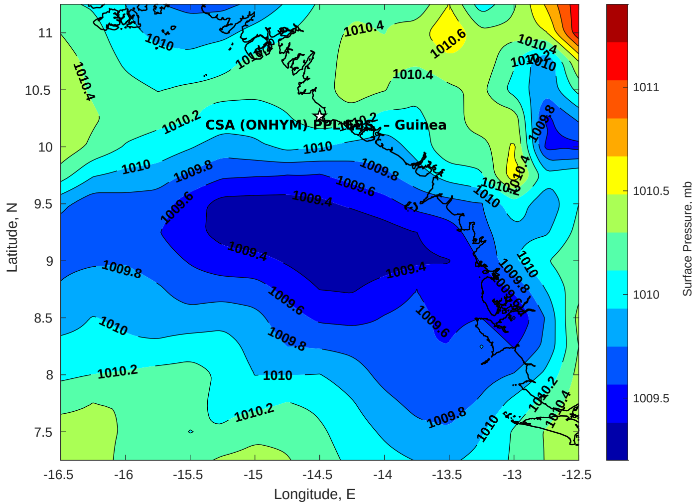
Surface Pressure (mb) for CSA (ONHYM) PPL EBS - Guinea at 23-Apr-2025 00:00:00
