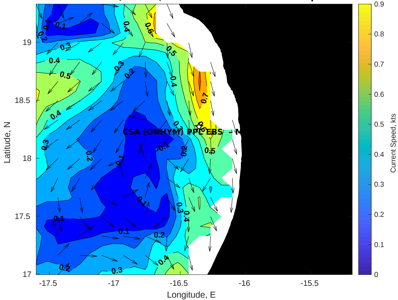
Surface Currents for CSA (ONHYM) PPL EBS - Mauritania at 20-Apr-2025 00:00:00
