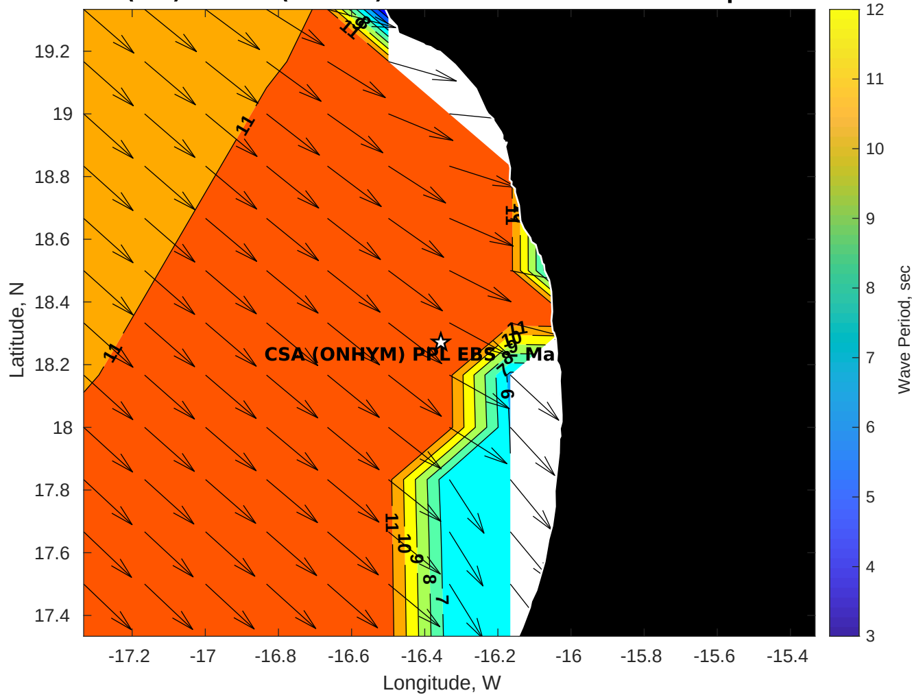
Wave Period (sec) for CSA (ONHYM) PPL EBS - Mauritania at 21-Apr-2025 09:00:00
