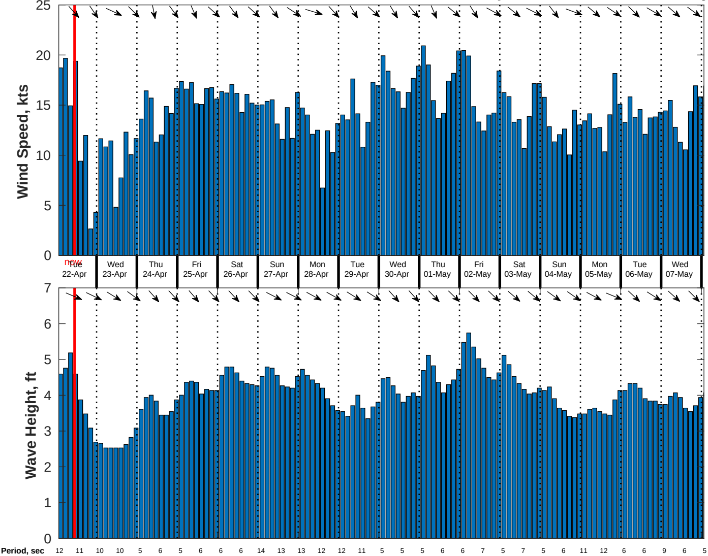
Wind & Wave Forecast for CSA (ONHYM) PPL EBS - Mauritania from 21-Apr-2025 01:00:00 to 07-May-2025 01:00:00
