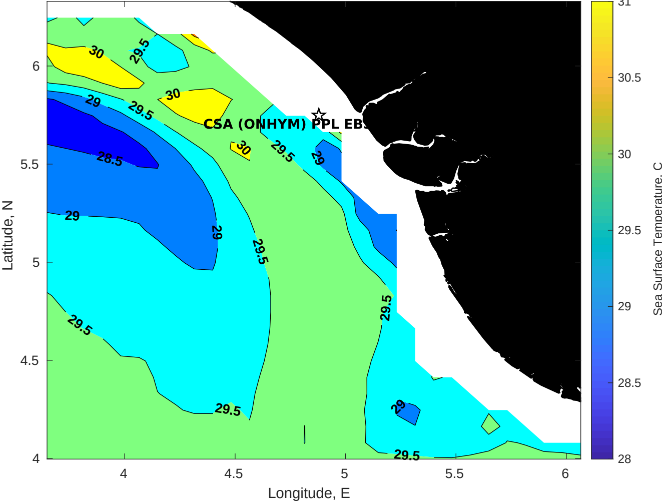
SST for CSA (ONHYM) PPL EBS - Nigeria at 20-Apr-2025 00:00:00
