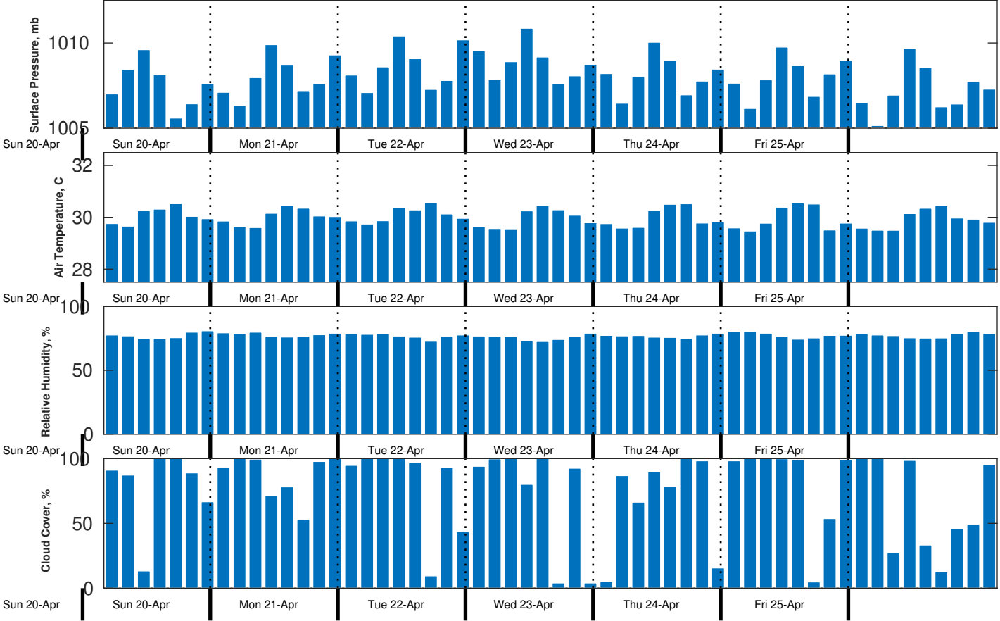
Met Forecast for CSA (ONHYM) PPL EBS - Nigeria from 21-Apr-2025 00:00:00 to 28-Apr-2025 00:00:00
