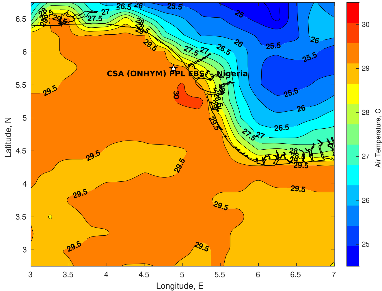
Air Temperature (C) for CSA (ONHYM) PPL EBS - Nigeria at 21-Apr-2025
