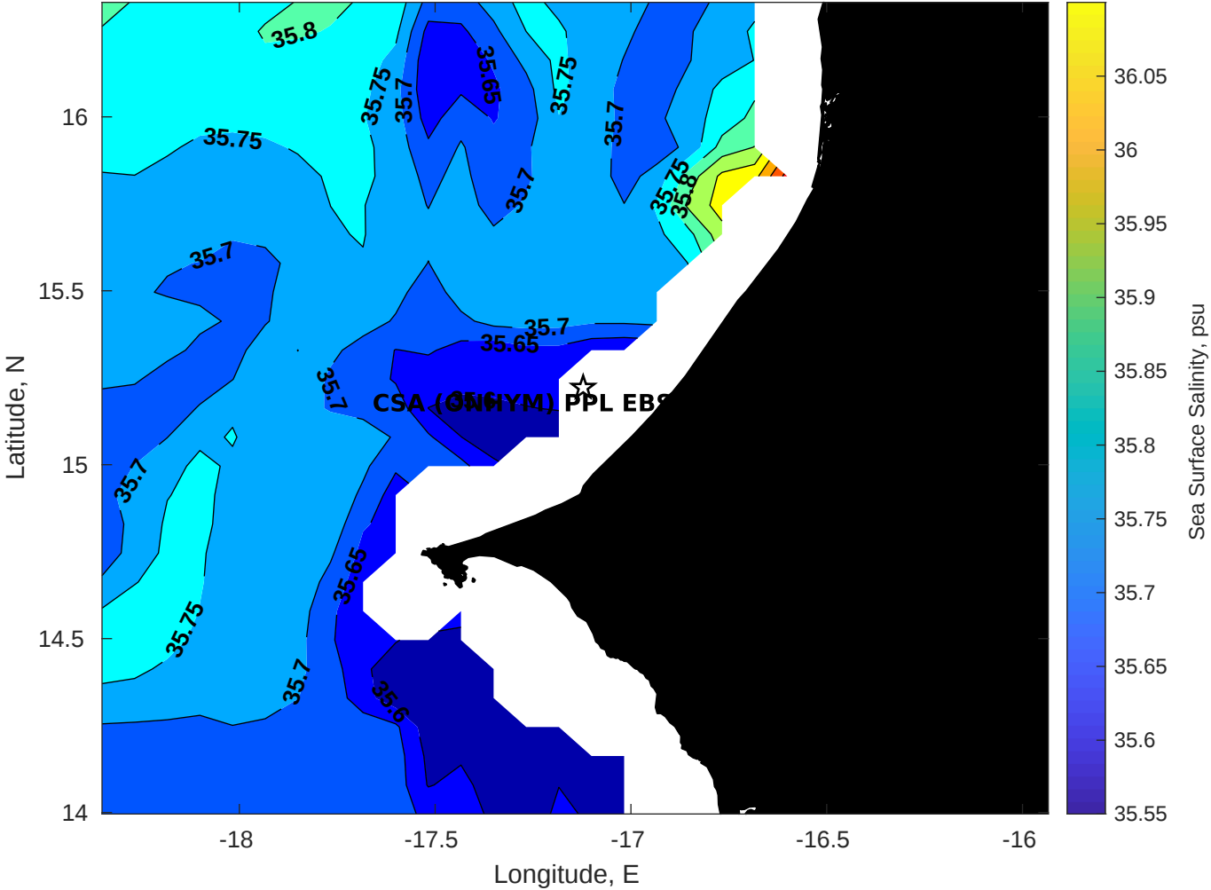
Surface Salinity for CSA (ONHYM) PPL EBS - Senegal at 20-Apr-2025 00:00:00
