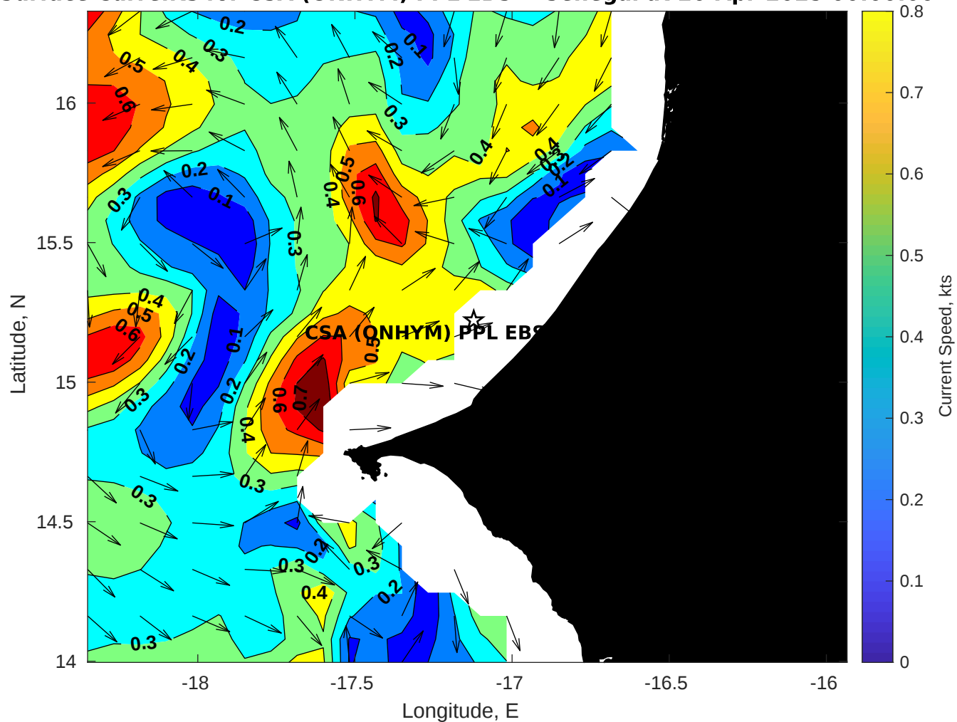
Surface Currents for CSA (ONHYM) PPL EBS - Senegal at 20-Apr-2025 00:00:00
