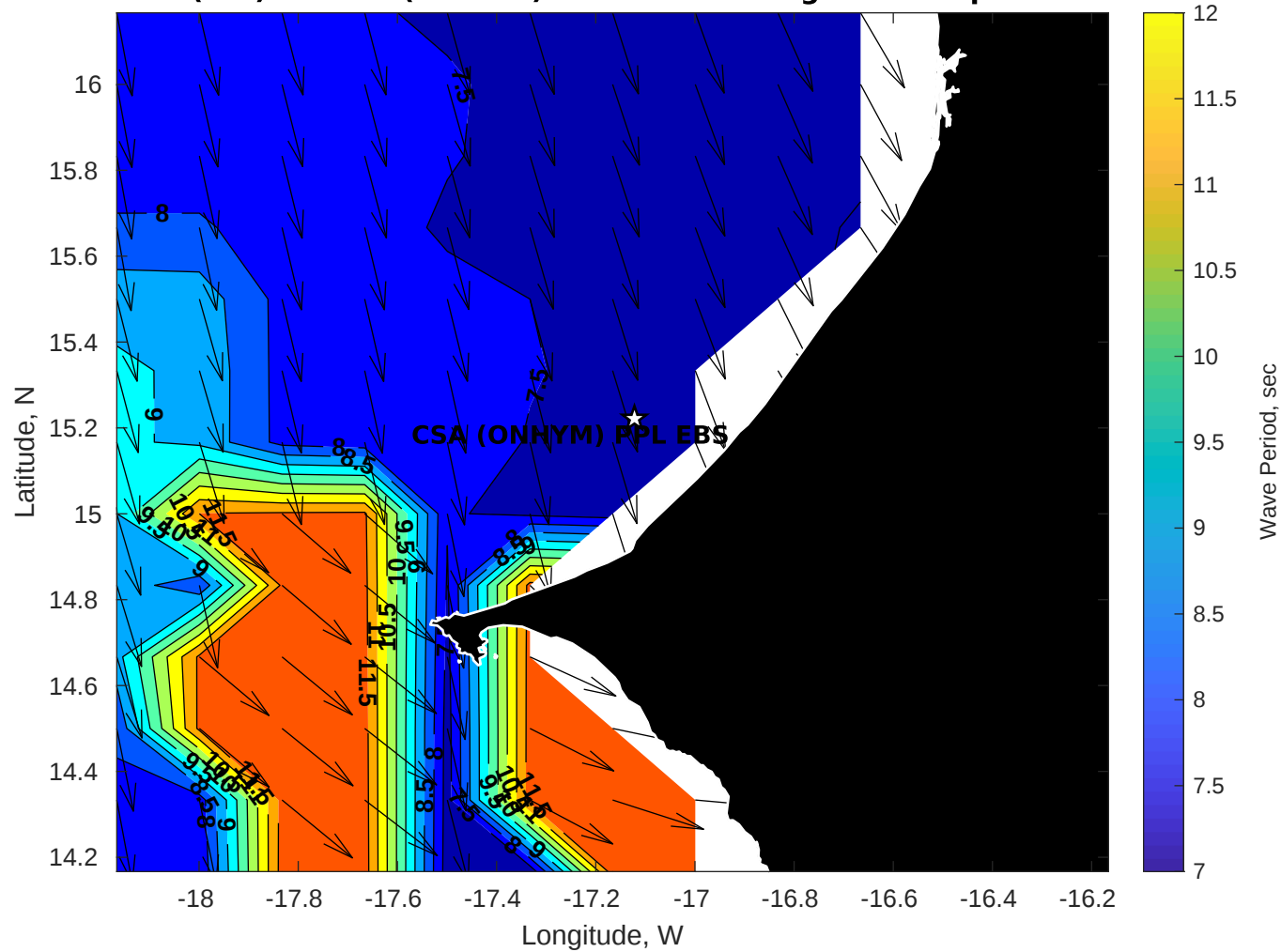
Wave Period (sec) for CSA (ONHYM) PPL EBS - Senegal at 21-Apr-2025 09:00:00
