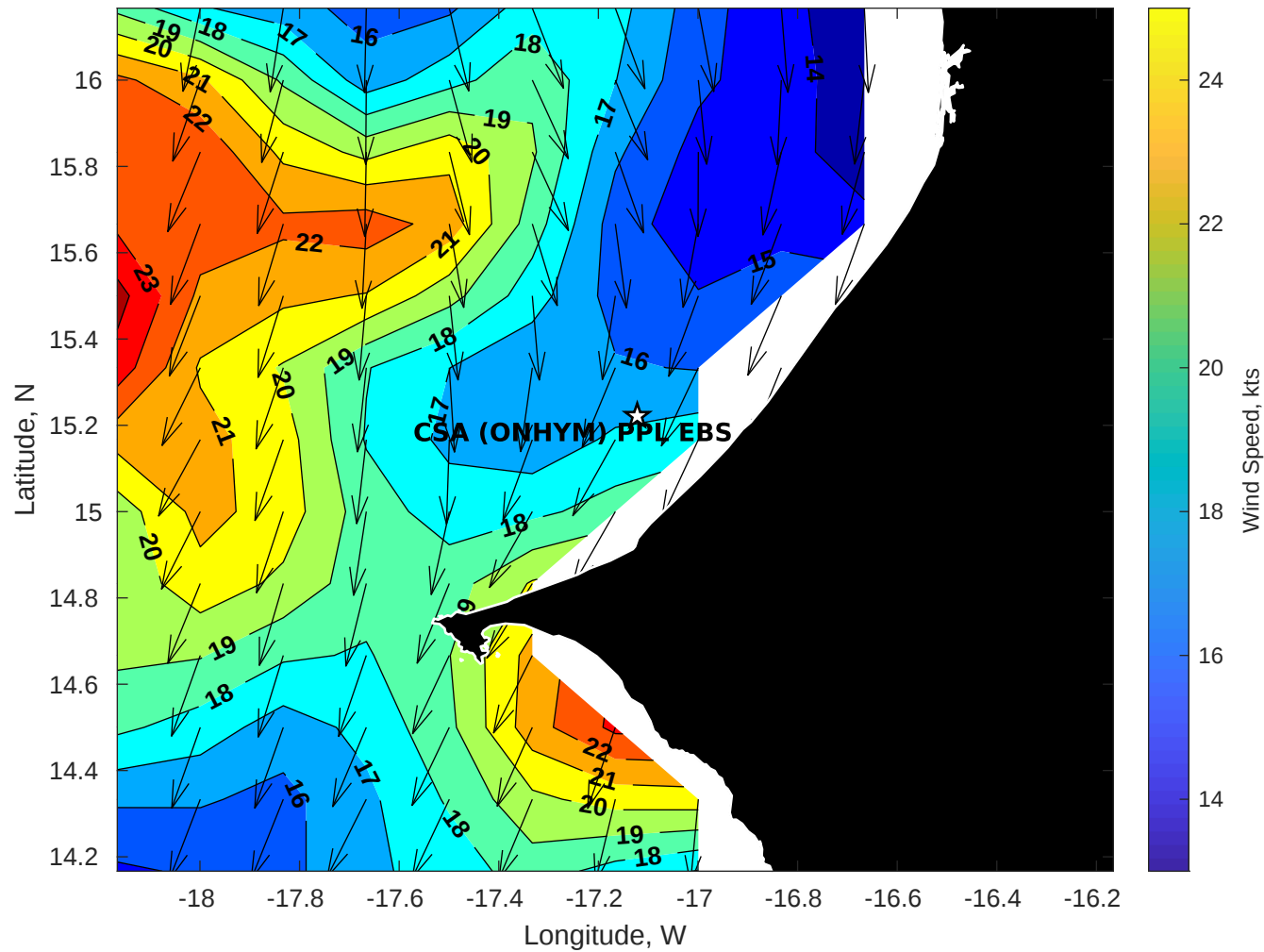
Winds (kts) for CSA (ONHYM) PPL EBS - Senegal at 21-Apr-2025 09:00:00
