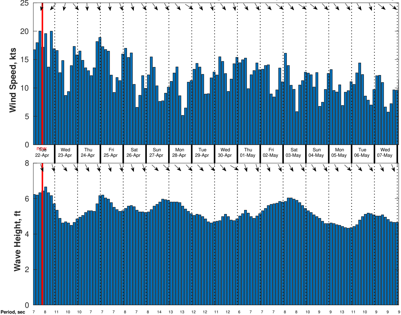
Wind & Wave Forecast for CSA (ONHYM) PPL EBS - Senegal from 21-Apr-2025 01:00:00 to 07-May-2025 01:00:00
