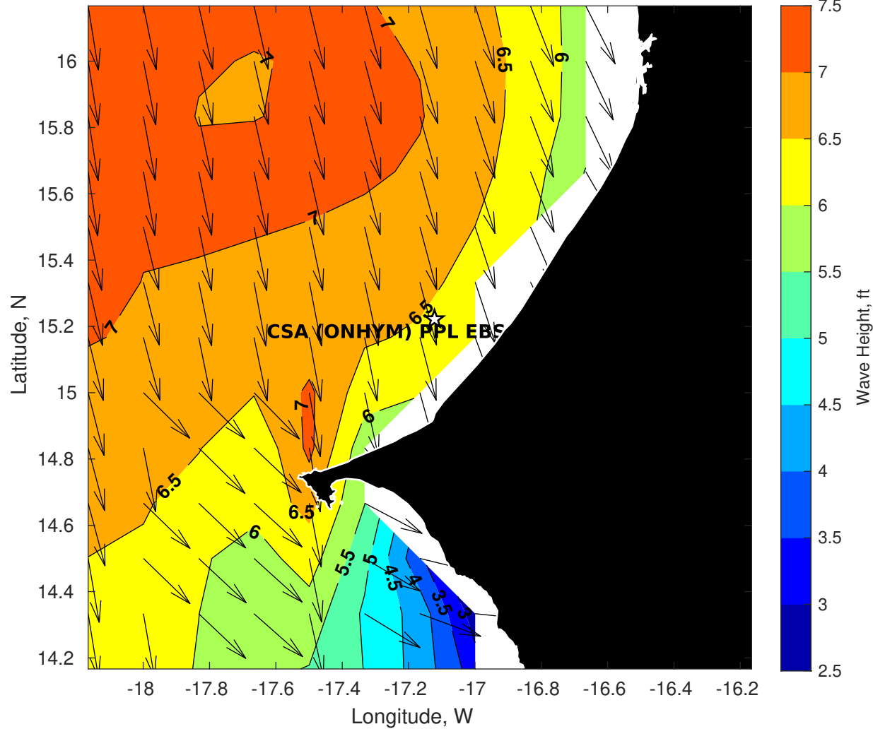
Wave Height (ft) for CSA (ONHYM) PPL EBS - Senegal at 21-Apr-2025 09:00:00
