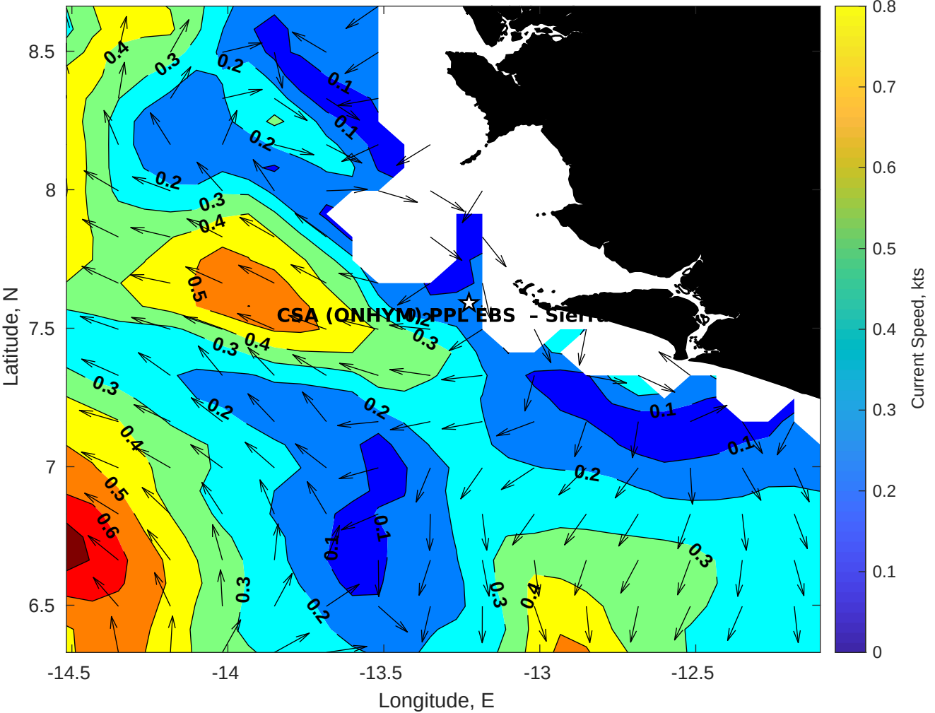
Surface Currents for CSA (ONHYM) PPL EBS - Sierra Leone at 20-Apr-2025 00:00:00
