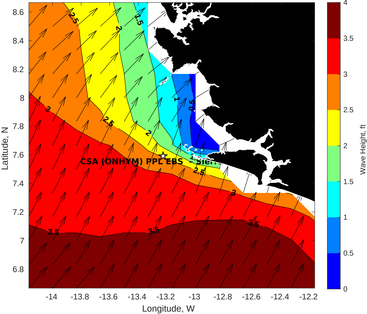
Wave Height (ft) for CSA (ONHYM) PPL EBS - Sierra Leone at 21-Apr-2025 09:00:00
