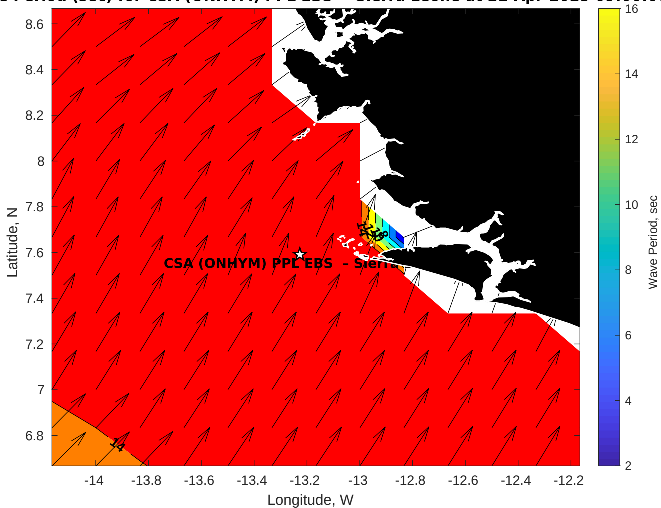
Wave Period (sec) for CSA (ONHYM) PPL EBS - Sierra Leone at 21-Apr-2025 09:00:00
