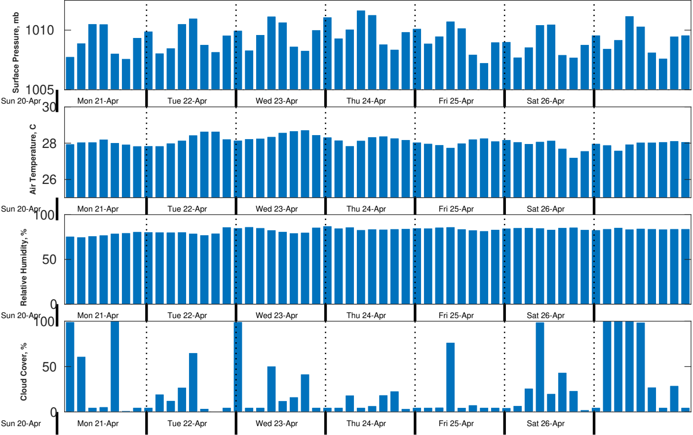
Met Forecast for CSA (ONHYM) PPL EBS - Sierra Leone from 21-Apr-2025 00:00:00 to 28-Apr-2025 00:00:00
