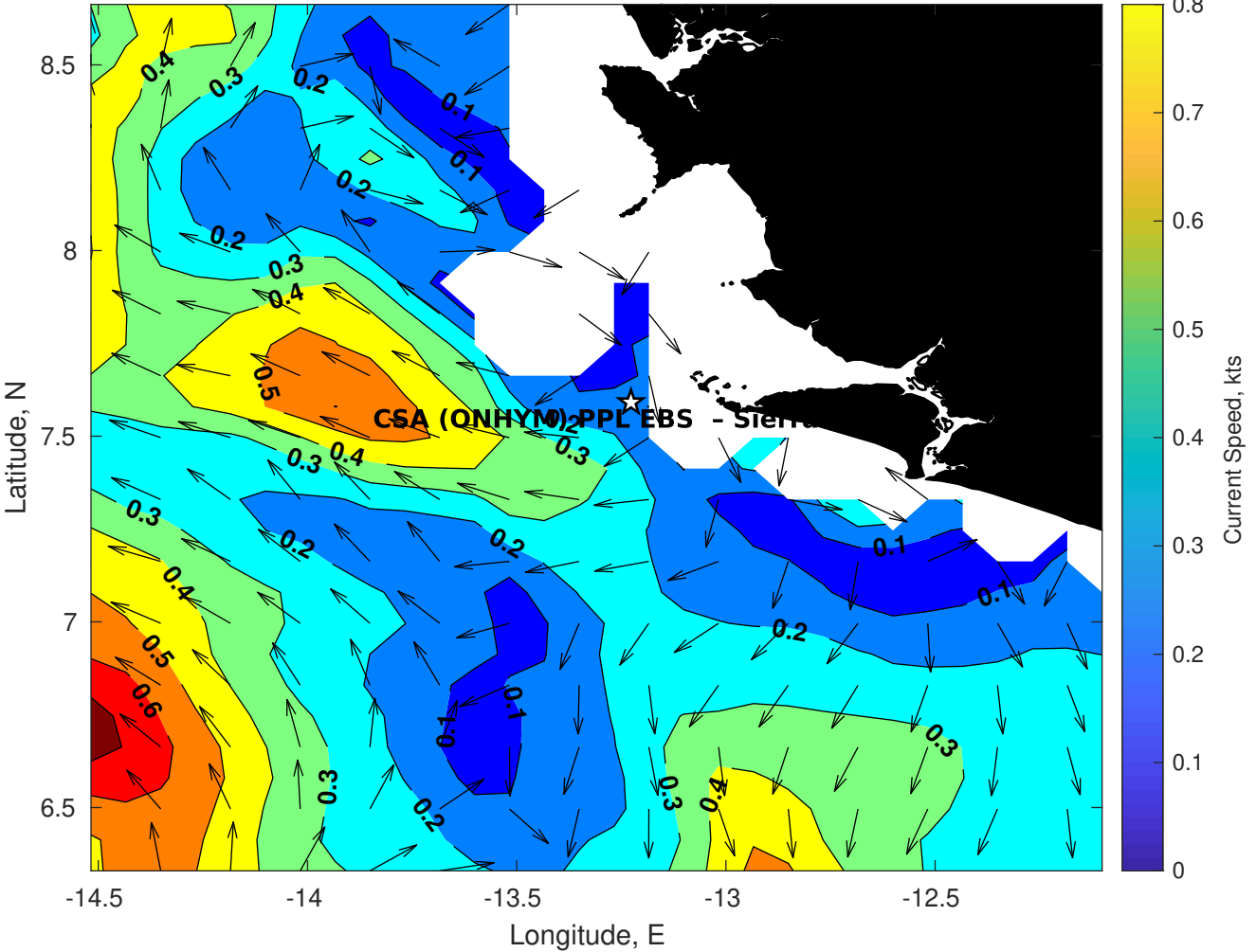
Surface Currents for CSA (ONHYM) PPL EBS - Sierra Leone at 20-Apr-2025 00:00:00
