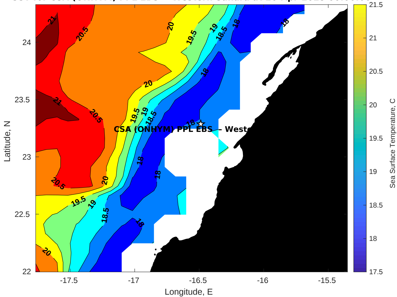
SST for CSA (ONHYM) PPL EBS - Western Sahara at 20-Apr-2025 00:00:00
