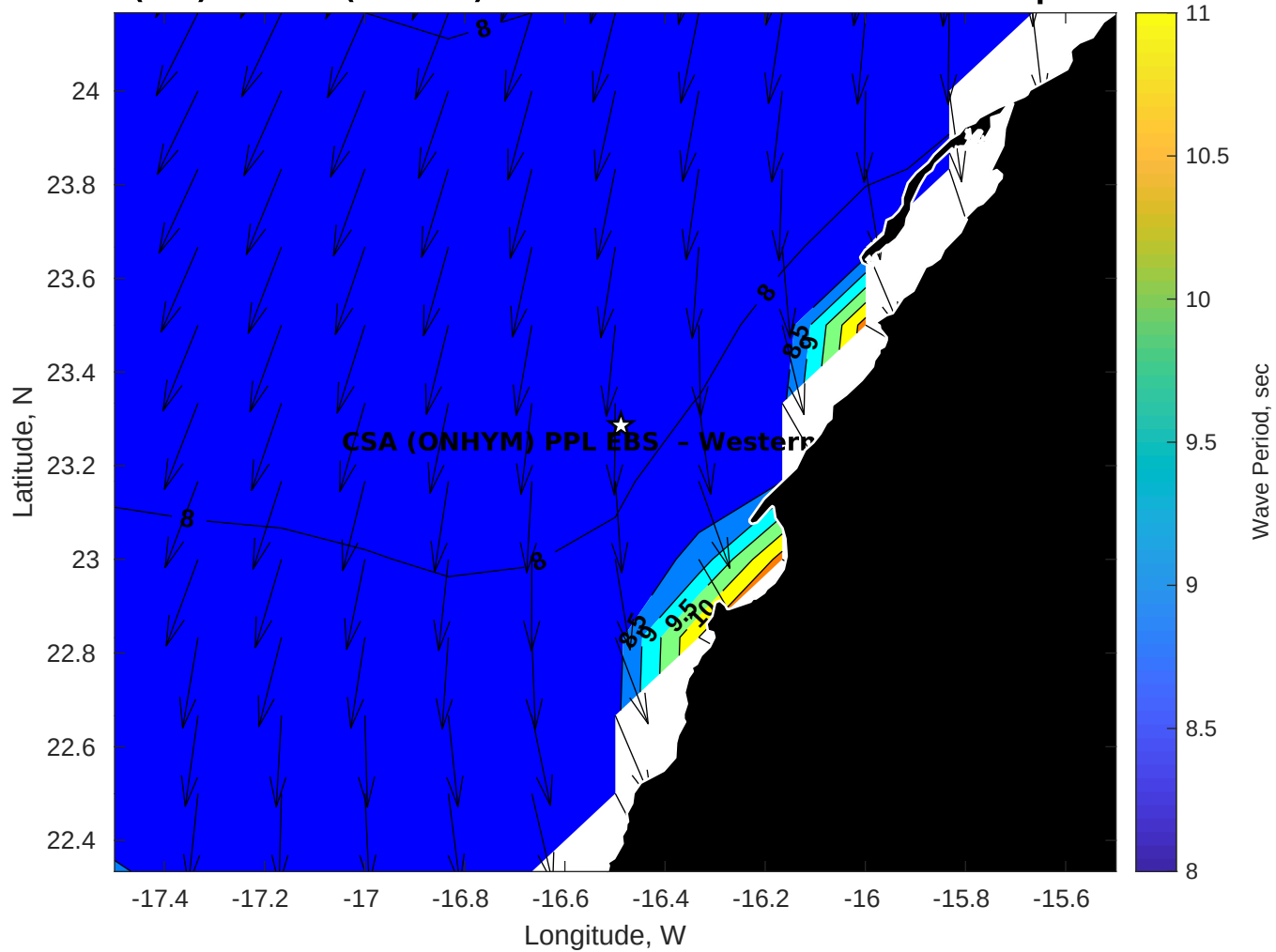
Wave Period (sec) for CSA (ONHYM) PPL EBS - Western Sahara at 21-Apr-2025 09:00:00
