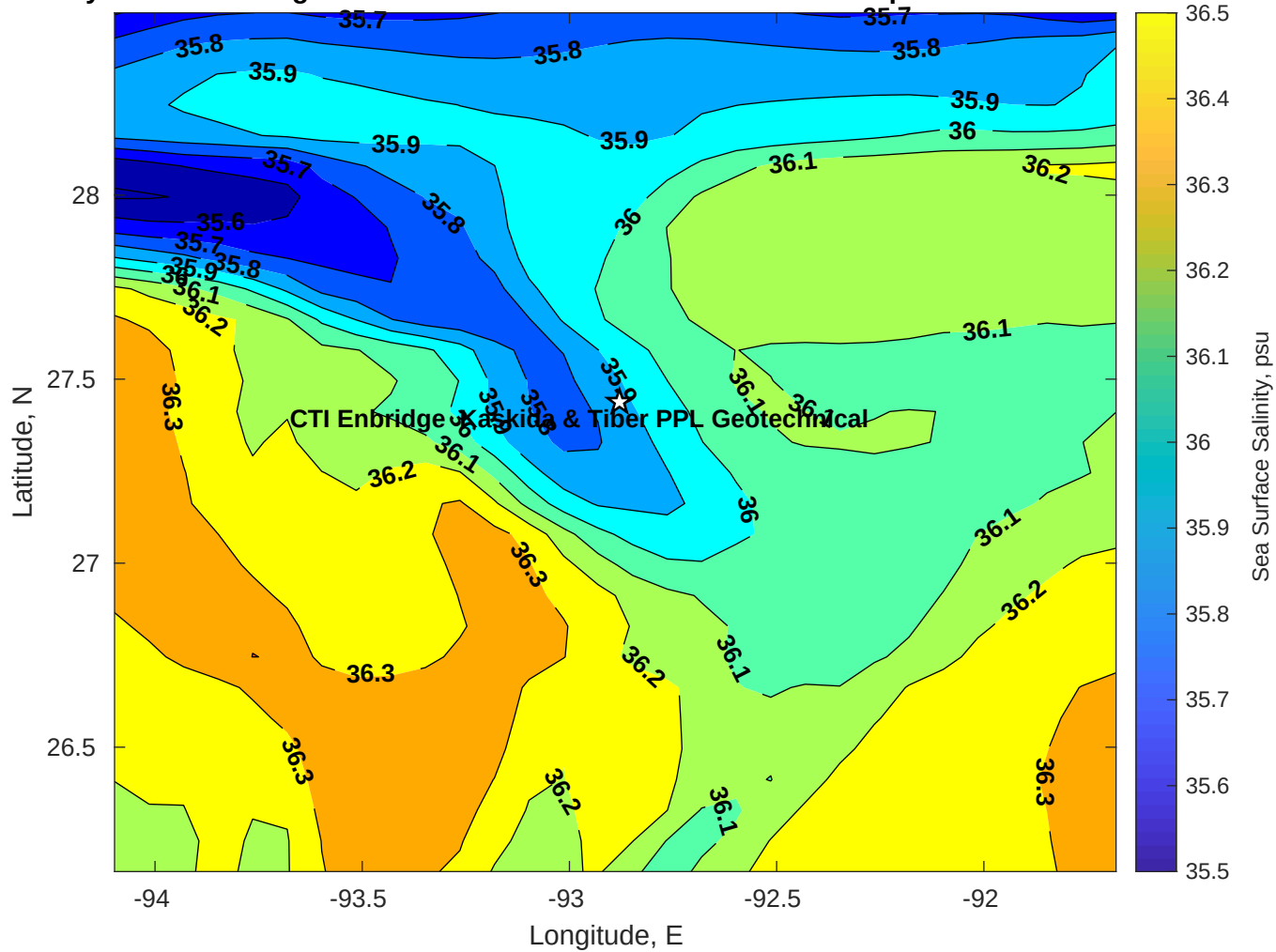
Surface Salinity for CTI Enbridge Kaskida & Tiber PPL Geotechnical at 20-Apr-2025 00:00:00
