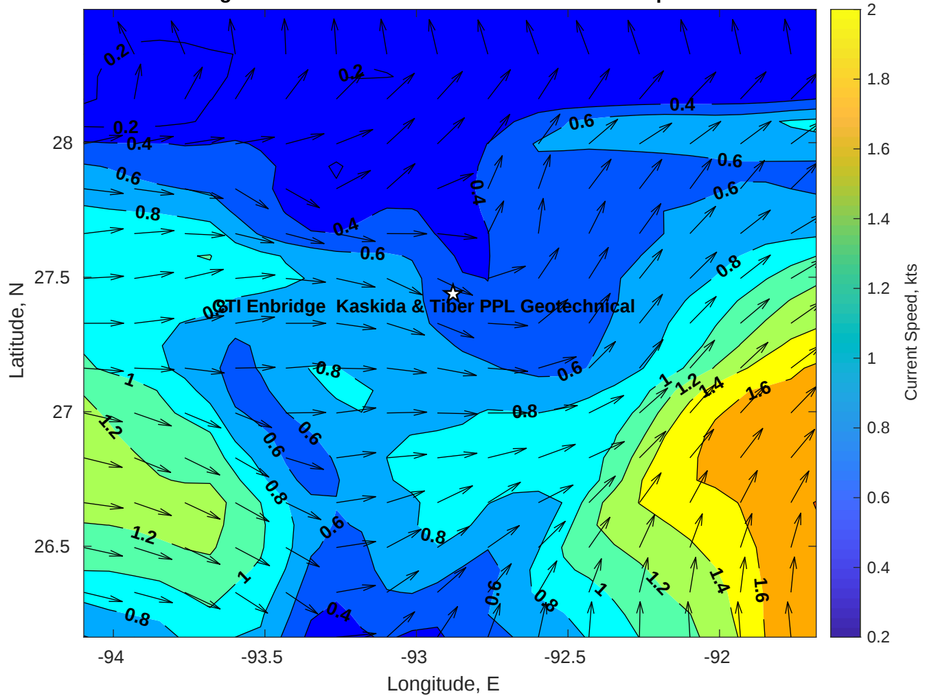
Surface Currents for CTI Enbridge Kaskida & Tiber PPL Geotechnical at 20-Apr-2025 00:00:00
