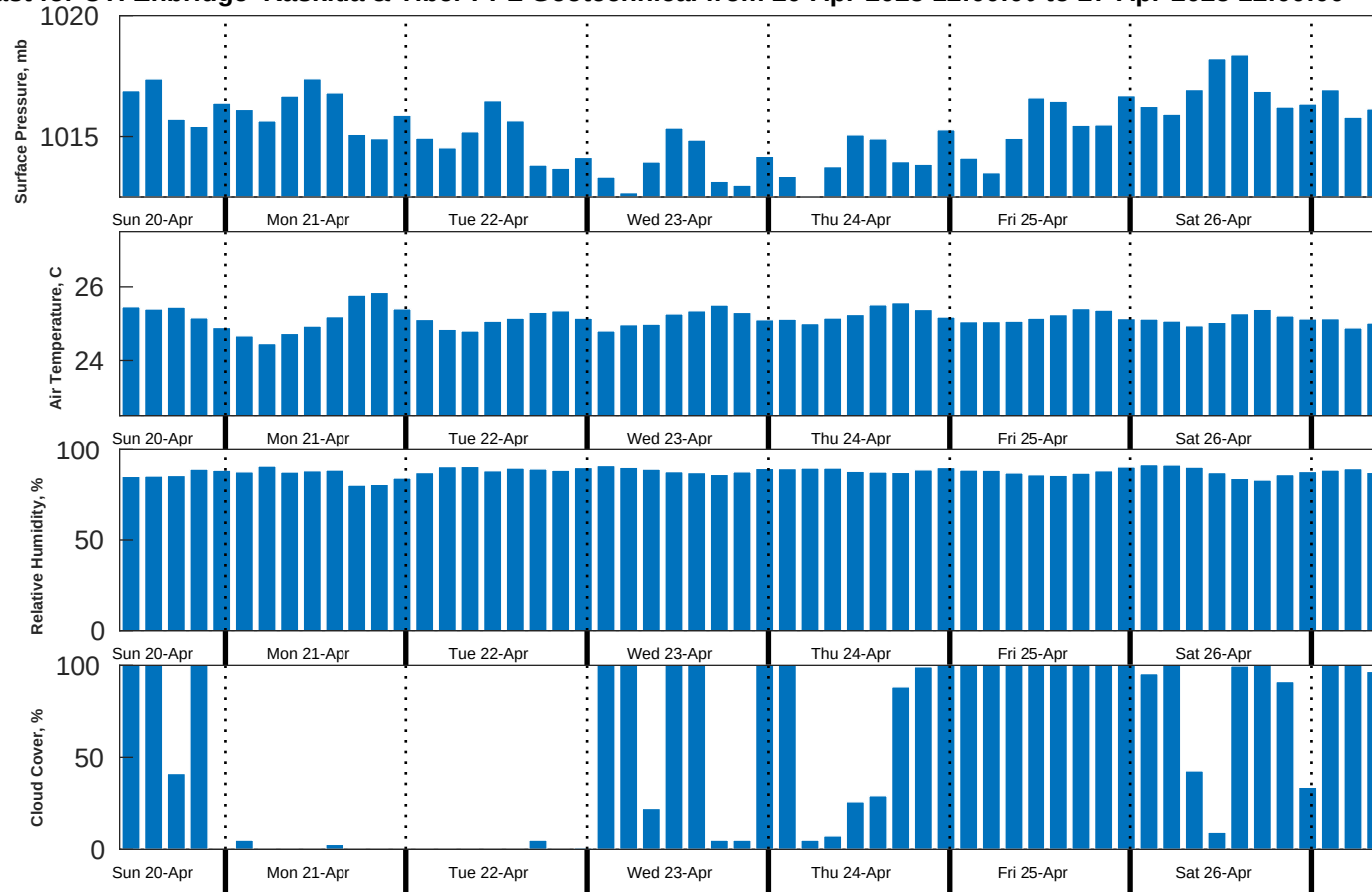
Met Forecast for CTI Enbridge Kaskida & Tiber PPL Geotechnical from 20-Apr-2025 12:00:00 to 27-Apr-2025 12:00:00
