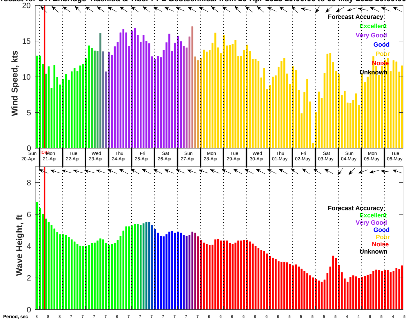
Wind & Wave Forecast for CTI Enbridge Kaskida & Tiber PPL Geotechnical from 20-Apr-2025 20:00:00 to 06-May-2025 20:00:00
