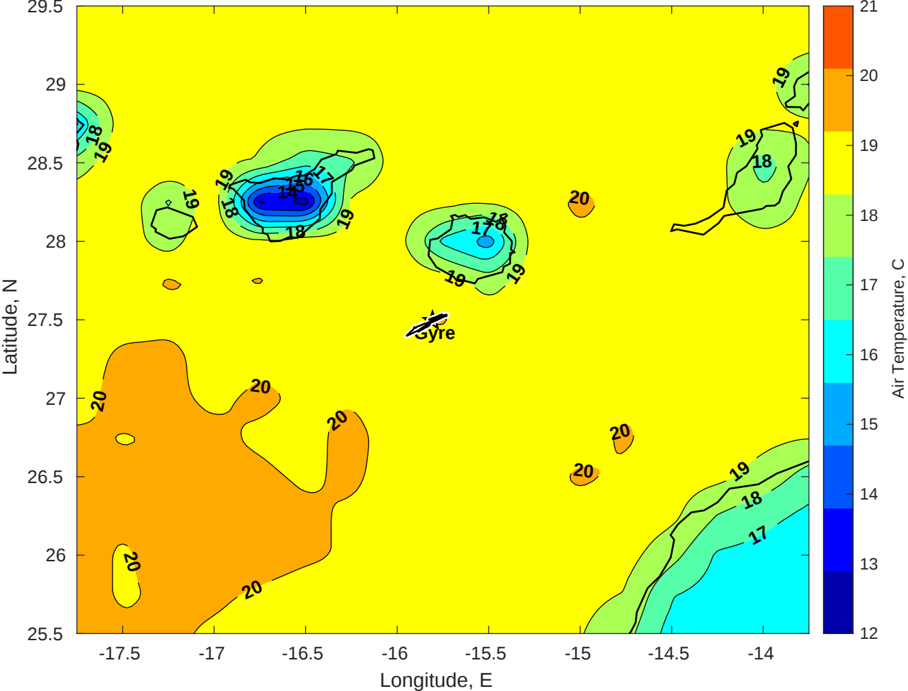
Air Temperature (C) for Gyre at 21-Apr-2025
