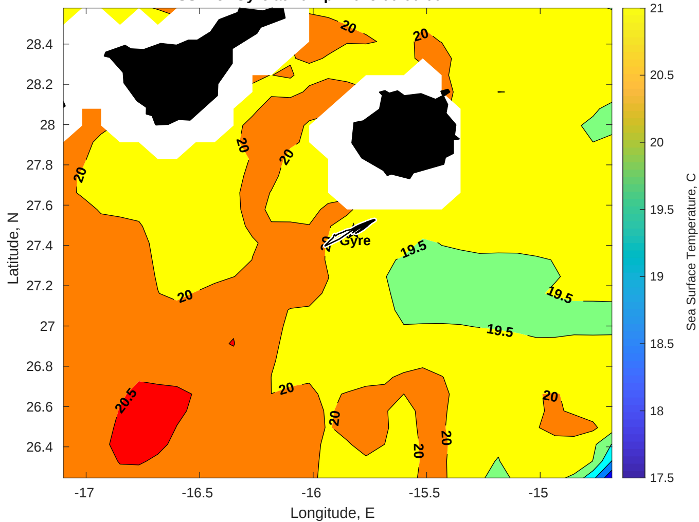
SST for Gyre at 20-Apr-2025 00:00:00
