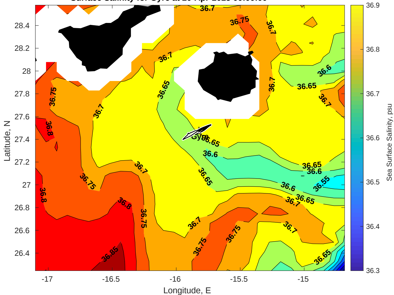
Surface Salinity for Gyre at 20-Apr-2025 00:00:00
