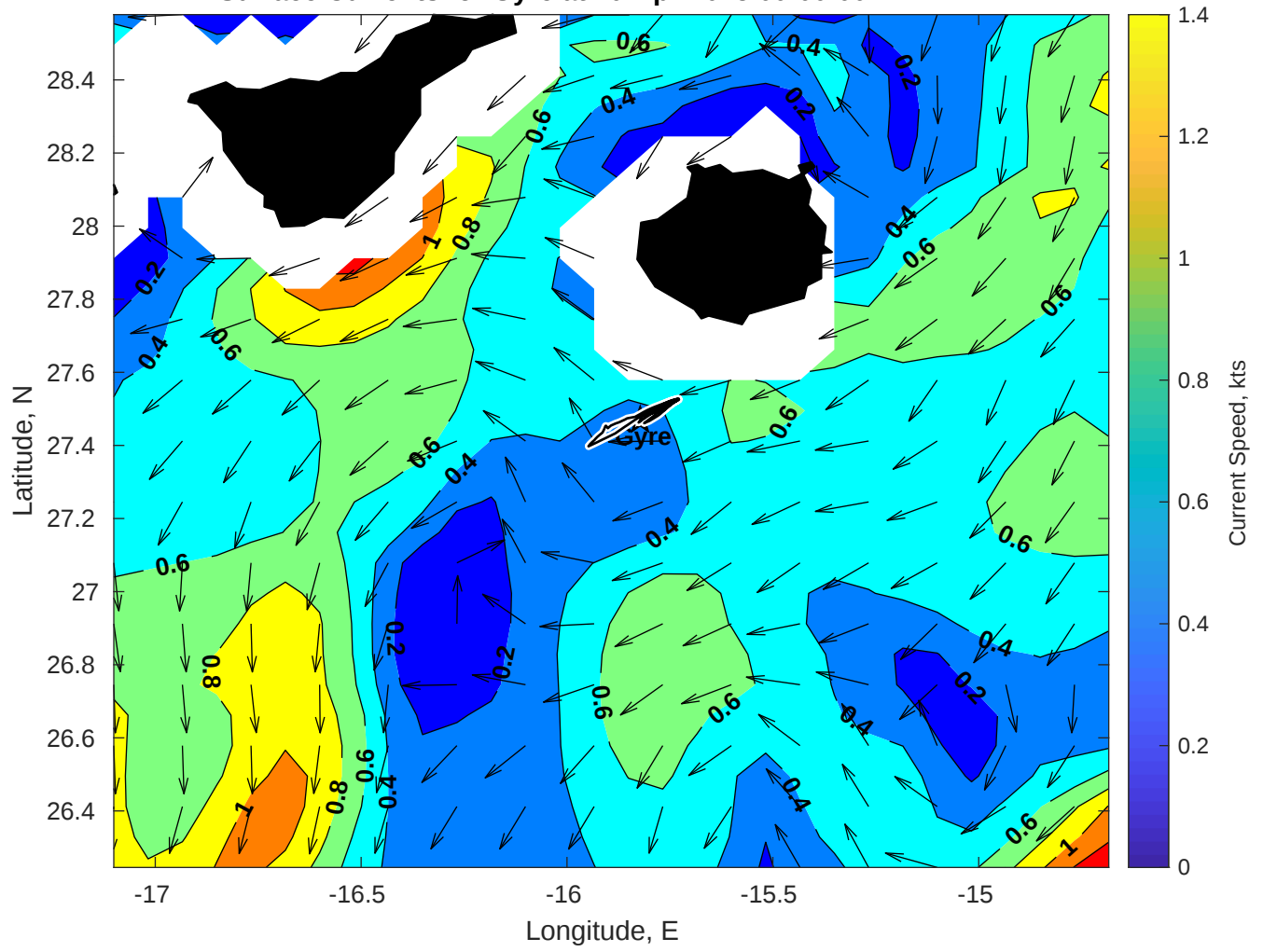
Surface Currents for Gyre at 20-Apr-2025 00:00:00
