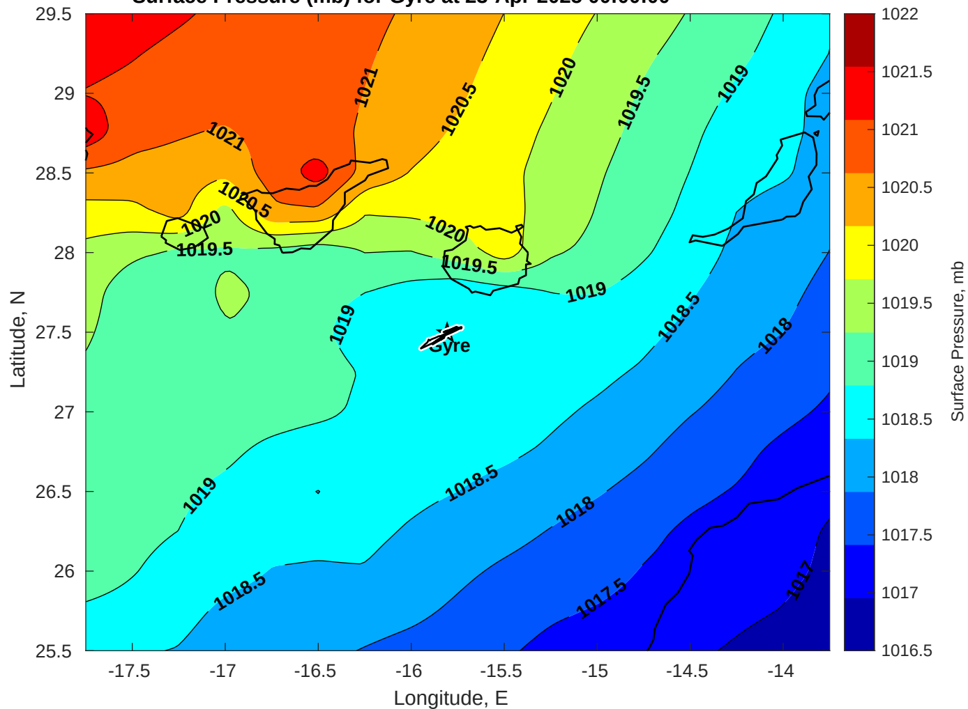
Surface Pressure (mb) for Gyre at 23-Apr-2025 00:00:00
