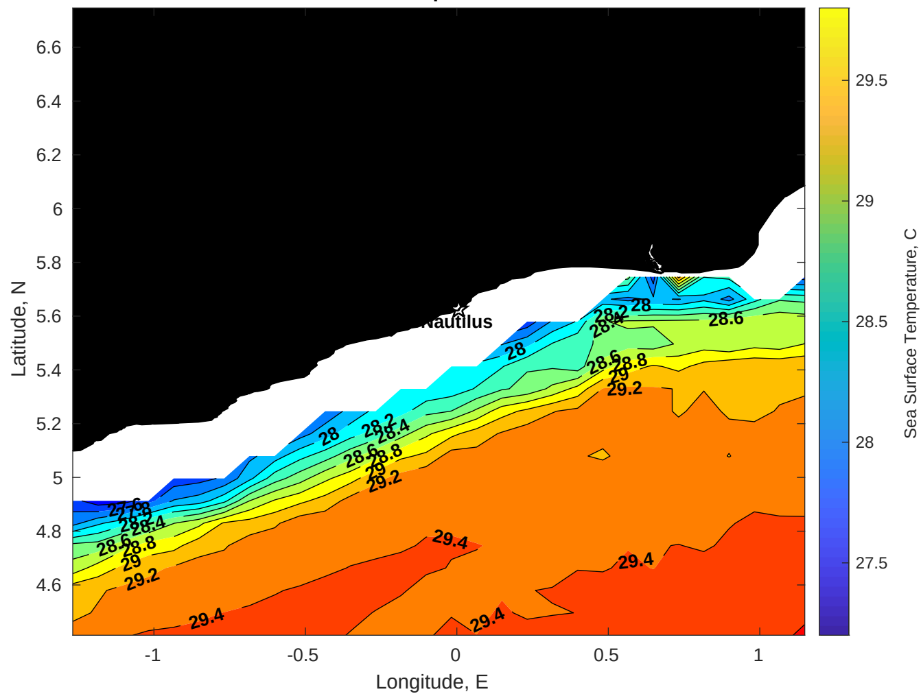
SST for Nautilus at 20-Apr-2025 00:00:00
