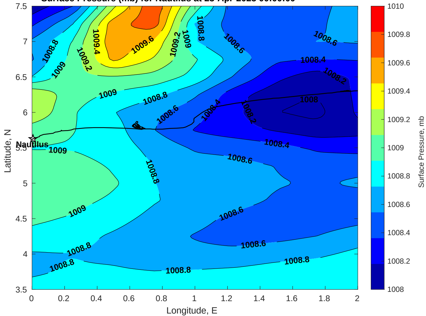
Surface Pressure (mb) for Nautilus at 23-Apr-2025 00:00:00
