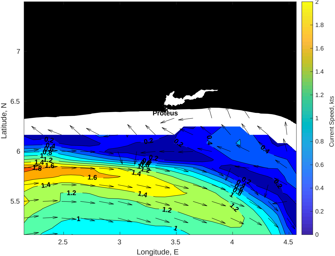
Surface Currents for Proteus at 20-Apr-2025 00:00:00
