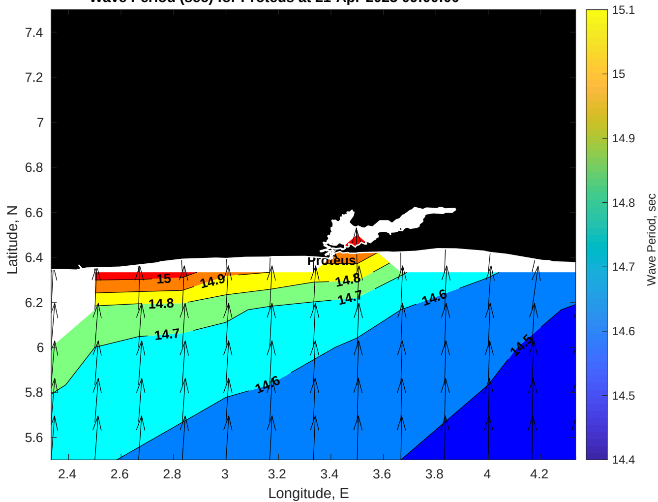
Wave Period (sec) for Proteus at 21-Apr-2025 09:00:00
