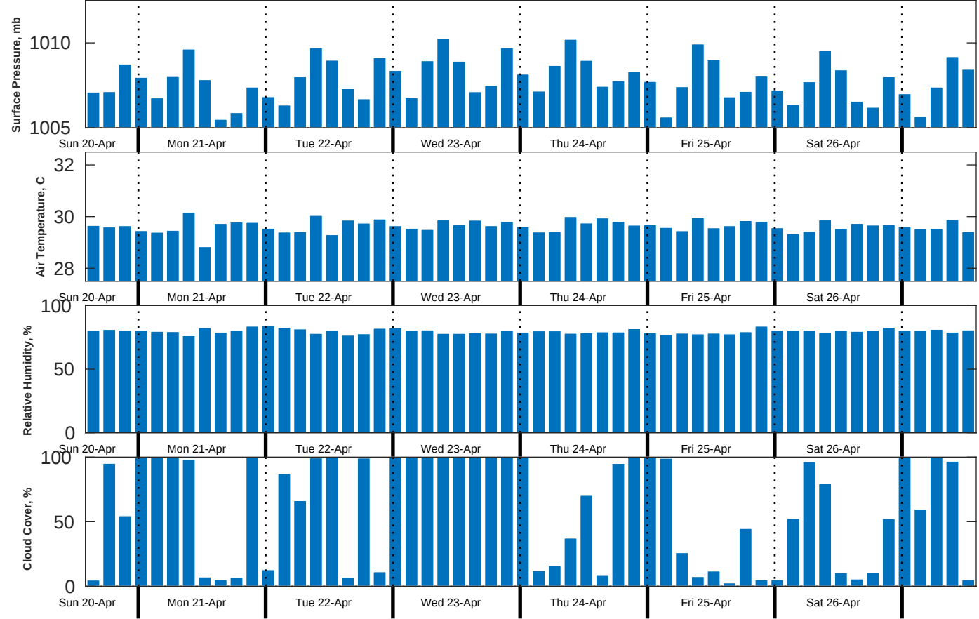
Met Forecast for Proteus from 20-Apr-2025 12:00:00 to 27-Apr-2025 12:00:00
