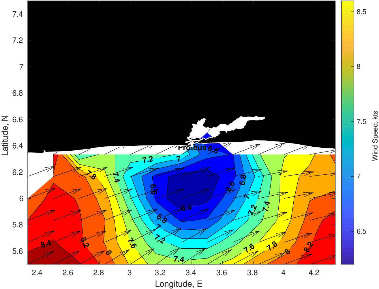
Winds (kts) for Proteus at 21-Apr-2025 09:00:00
