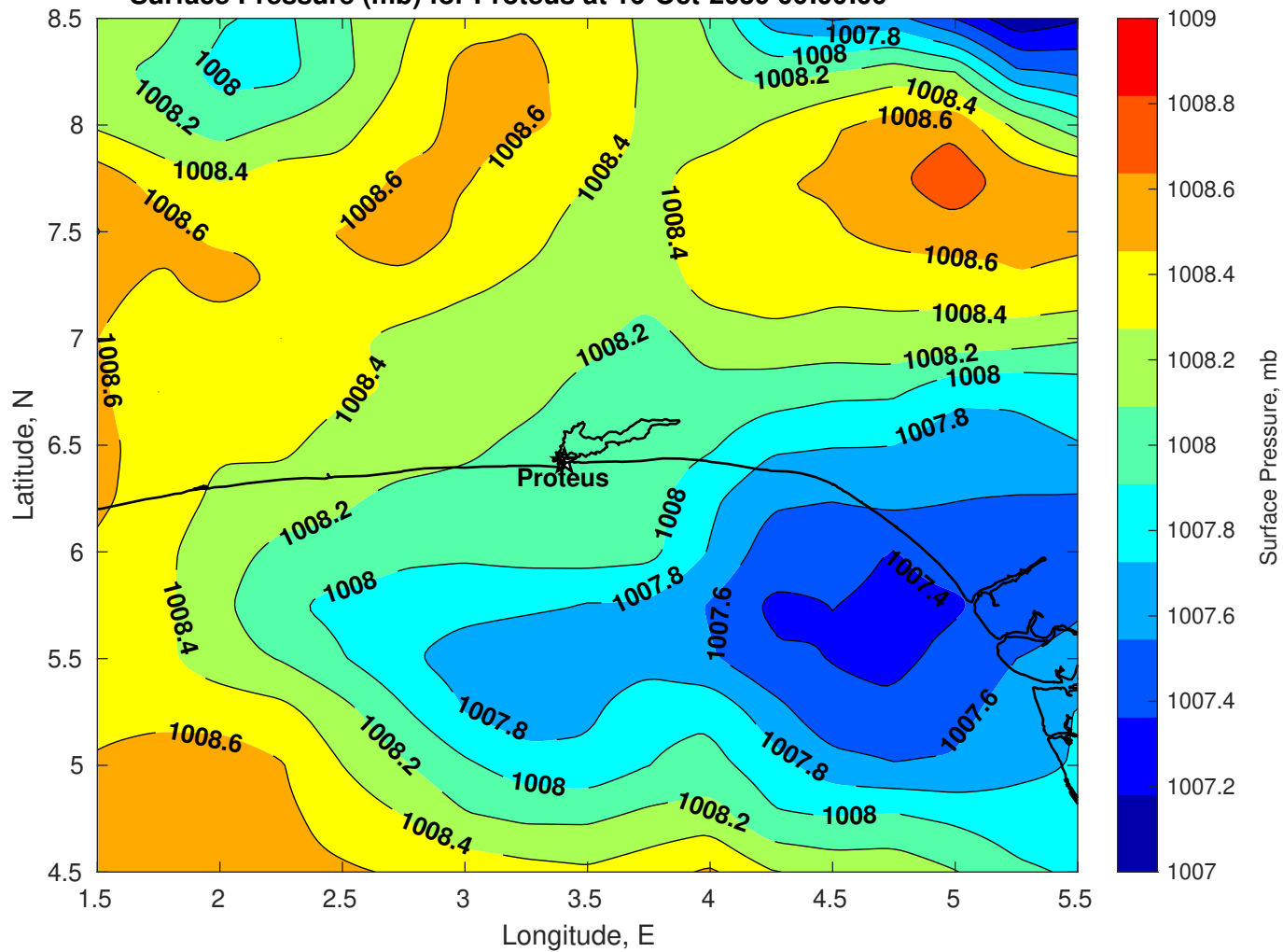
Surface Pressure (mb) for Proteus at 16-Oct-2030 00:00:00
