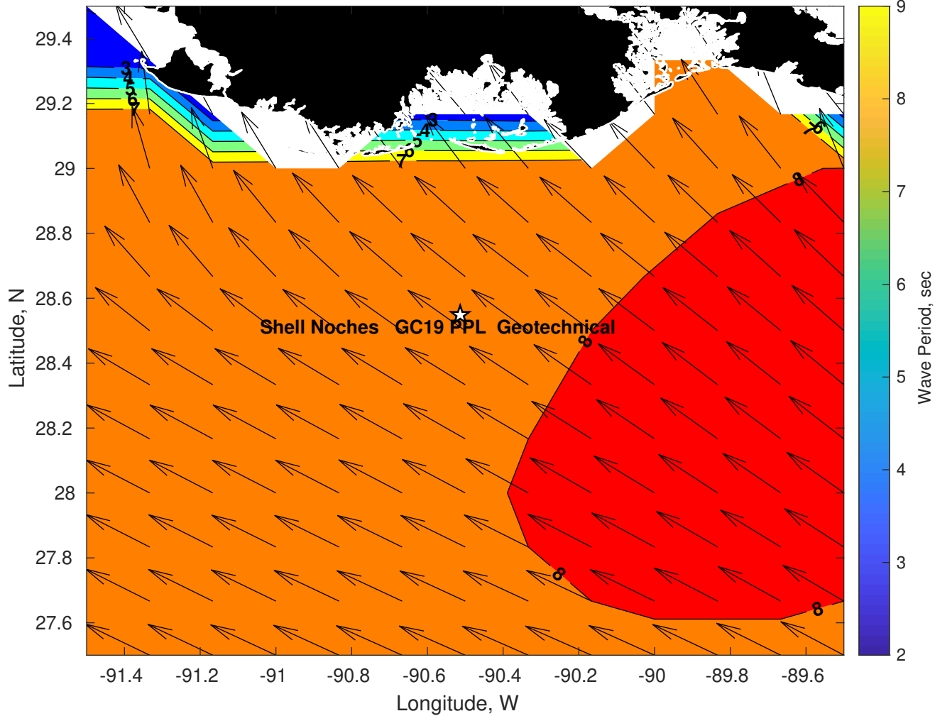
Wave Period (sec) for Shell Noches GC19 PPL Geotechnical at 21-Apr-2025 09:00:00
