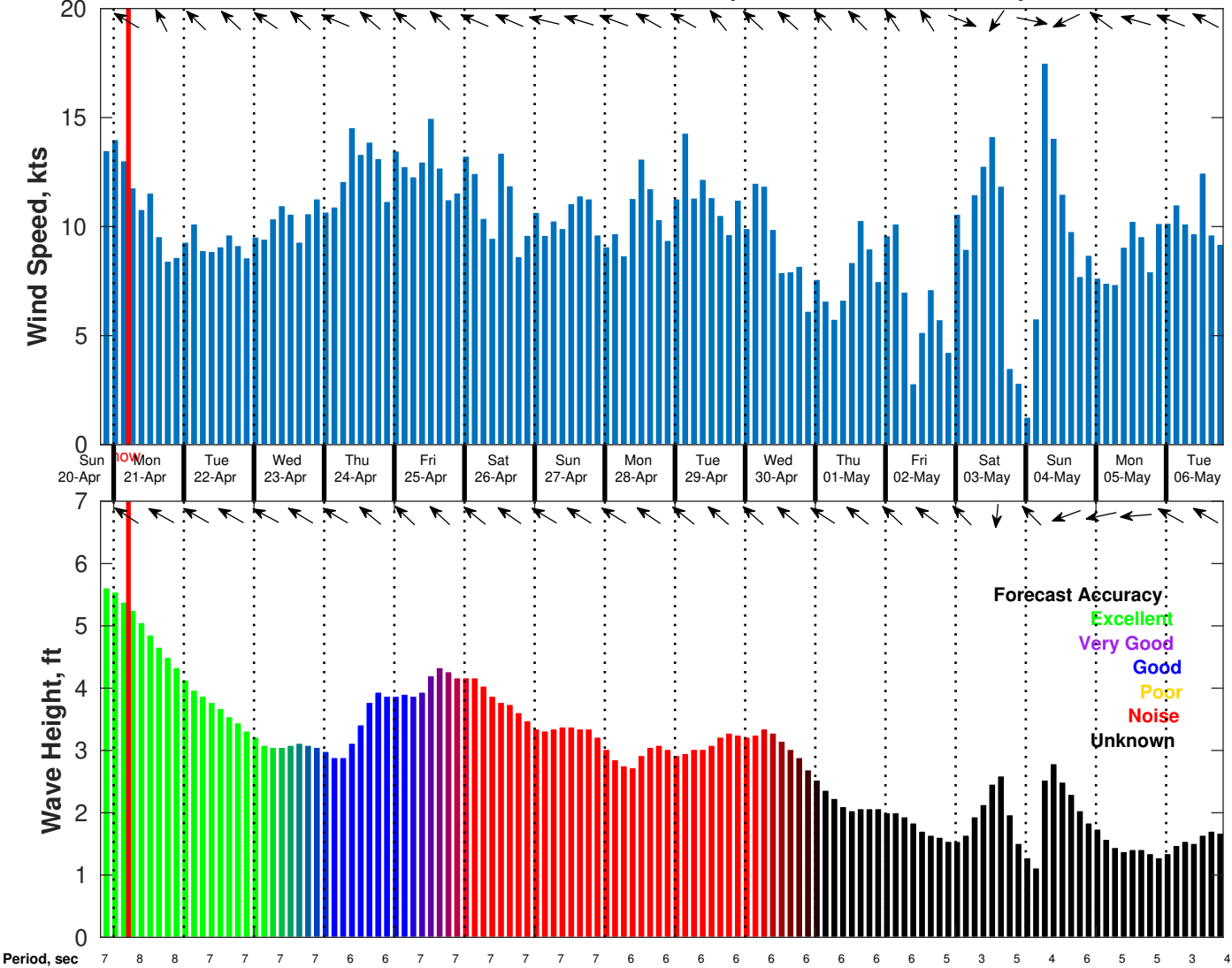
Wind & Wave Forecast for Shell Noches GC19 PPL Geotechnical from 20-Apr-2025 20:00:00 to 06-May-2025 20:00:00
