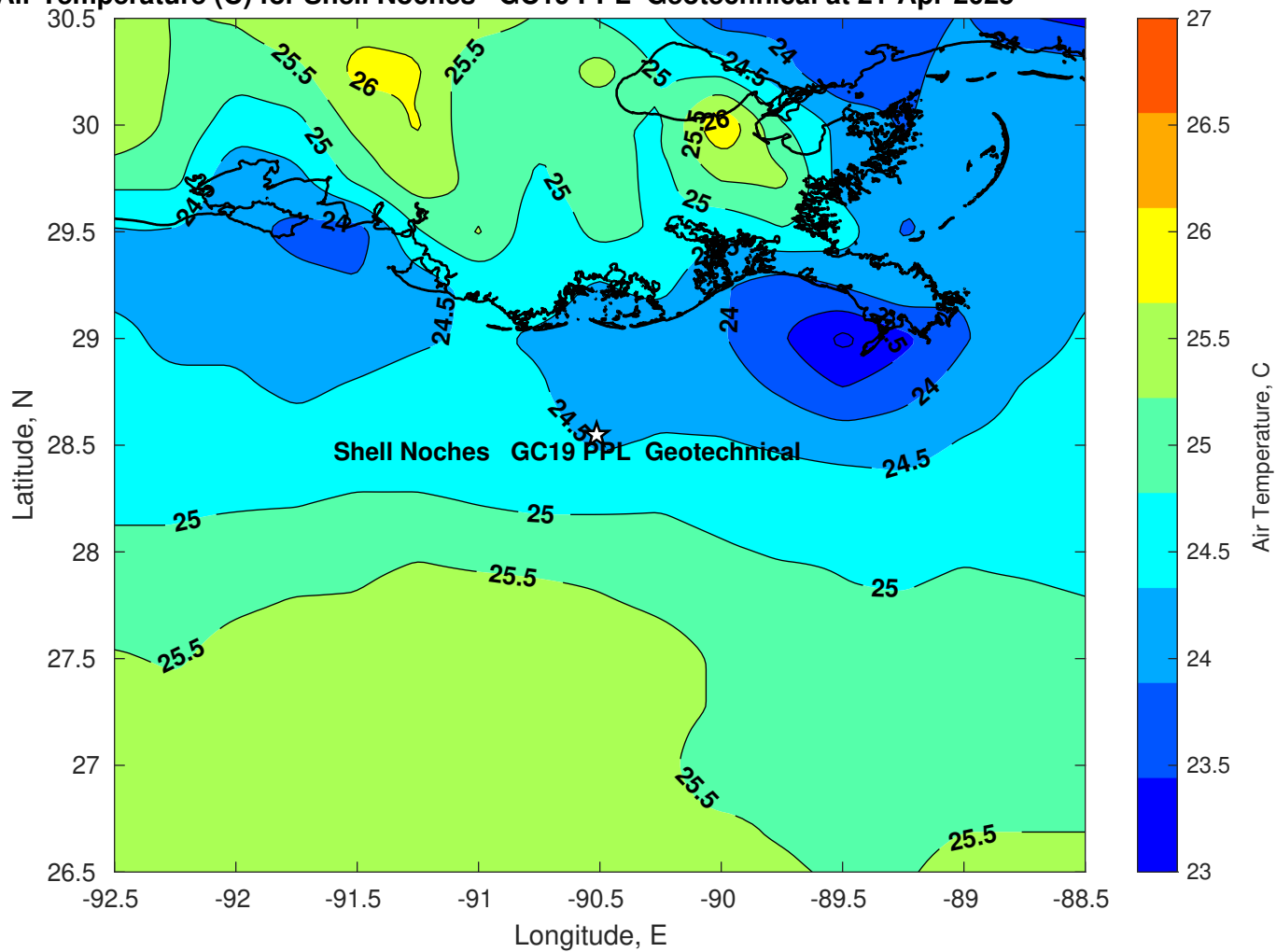
Air Temperature (C) for Shell Noches GC19 PPL Geotechnical at 21-Apr-2025
