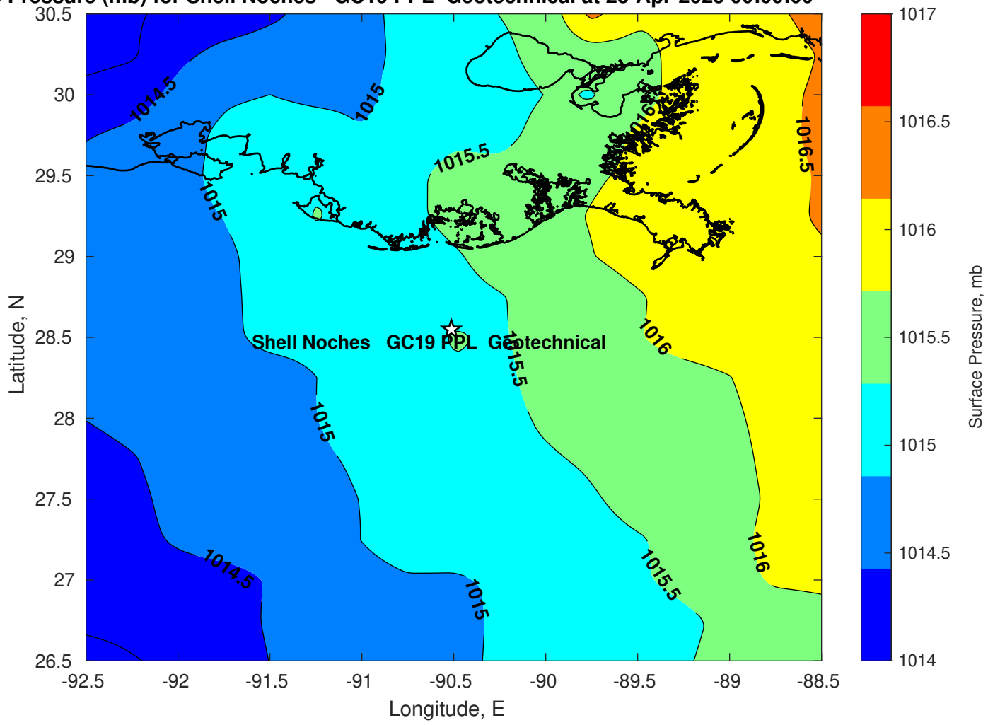
Surface Pressure (mb) for Shell Noches GC19 PPL Geotechnical at 23-Apr-2025 00:00:00
