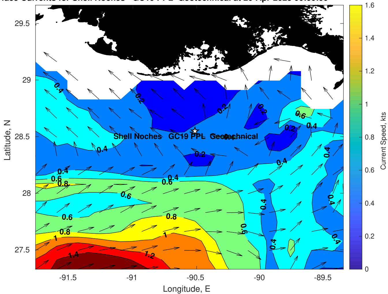
Surface Currents for Shell Noches GC19 PPL Geotechnical at 20-Apr-2025 00:00:00
