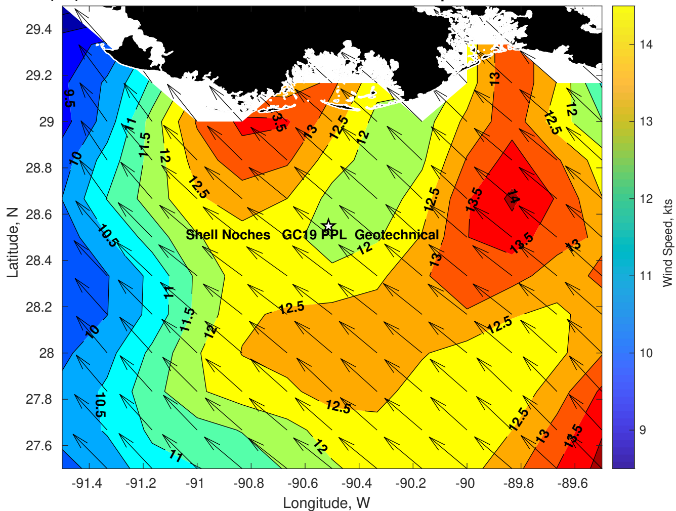
Winds (kts) for Shell Noches GC19 PPL Geotechnical at 21-Apr-2025 09:00:00
