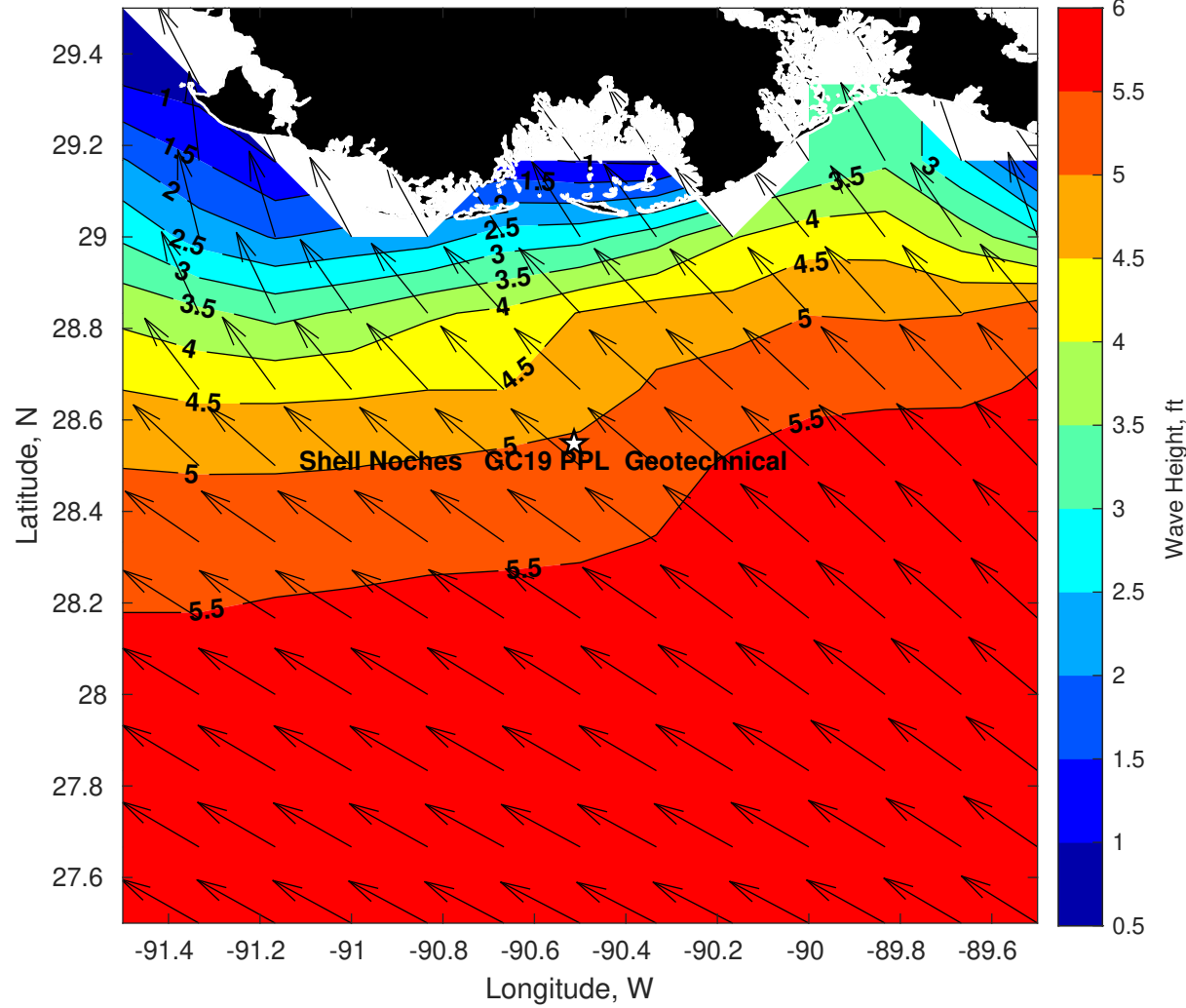
Wave Height (ft) for Shell Noches GC19 PPL Geotechnical at 21-Apr-2025 09:00:00
