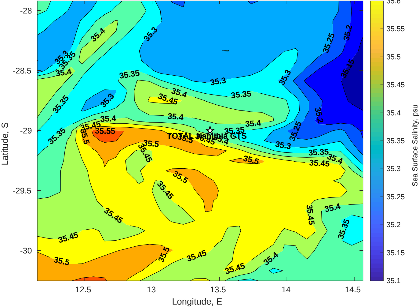
Surface Salinity for TOTAL Namibia GTS at 20-Apr-2025 00:00:00
