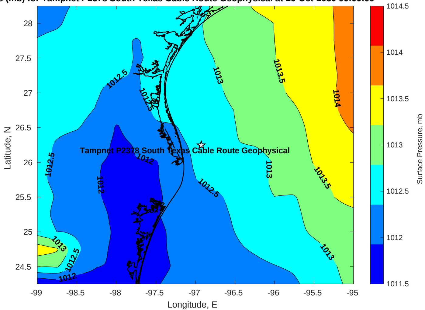
Pressure (mb) for Tampnet P2378 South Texas Cable Route Geophysical at 16-Oct-2030 00:00:00
