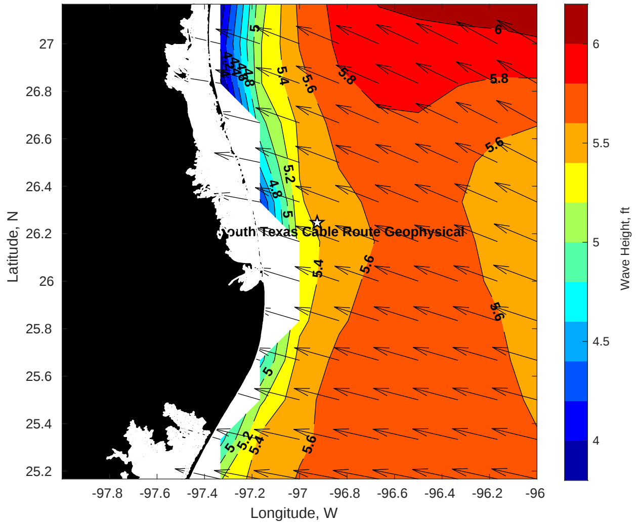
Wave Height (ft) for Tampnet P2378 South Texas Cable Route Geophysical at 21-Apr-2025 09:00:00
