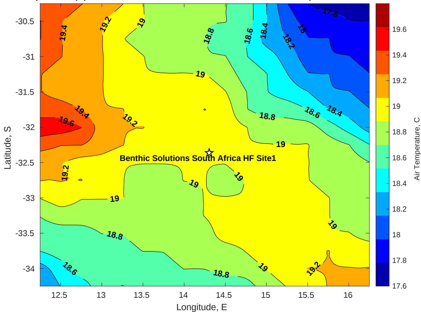
Air Temperature (C) for Benthic Solutions South Africa HF Site1 at 22-Apr-2025
