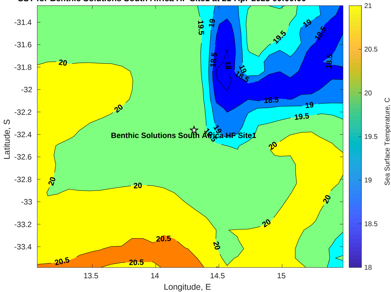
SST for Benthic Solutions South Africa HF Site1 at 21-Apr-2025 00:00:00
