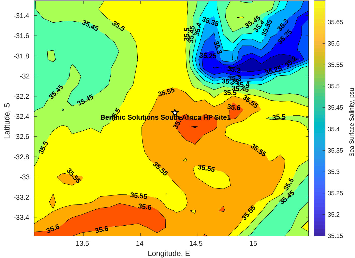
Surface Salinity for Benthic Solutions South Africa HF Site1 at 21-Apr-2025 00:00:00
